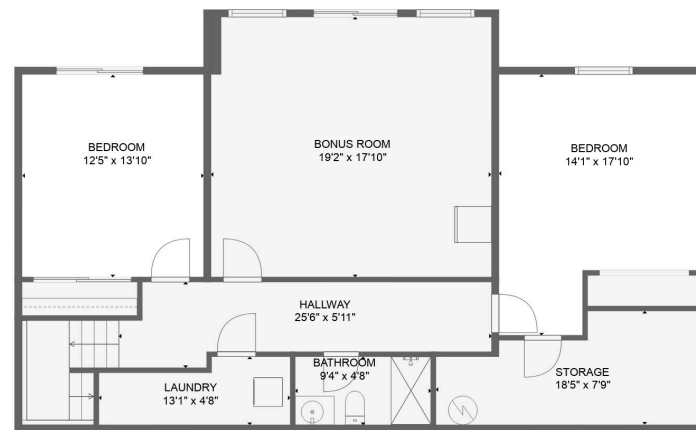
LOWER LEVEL
