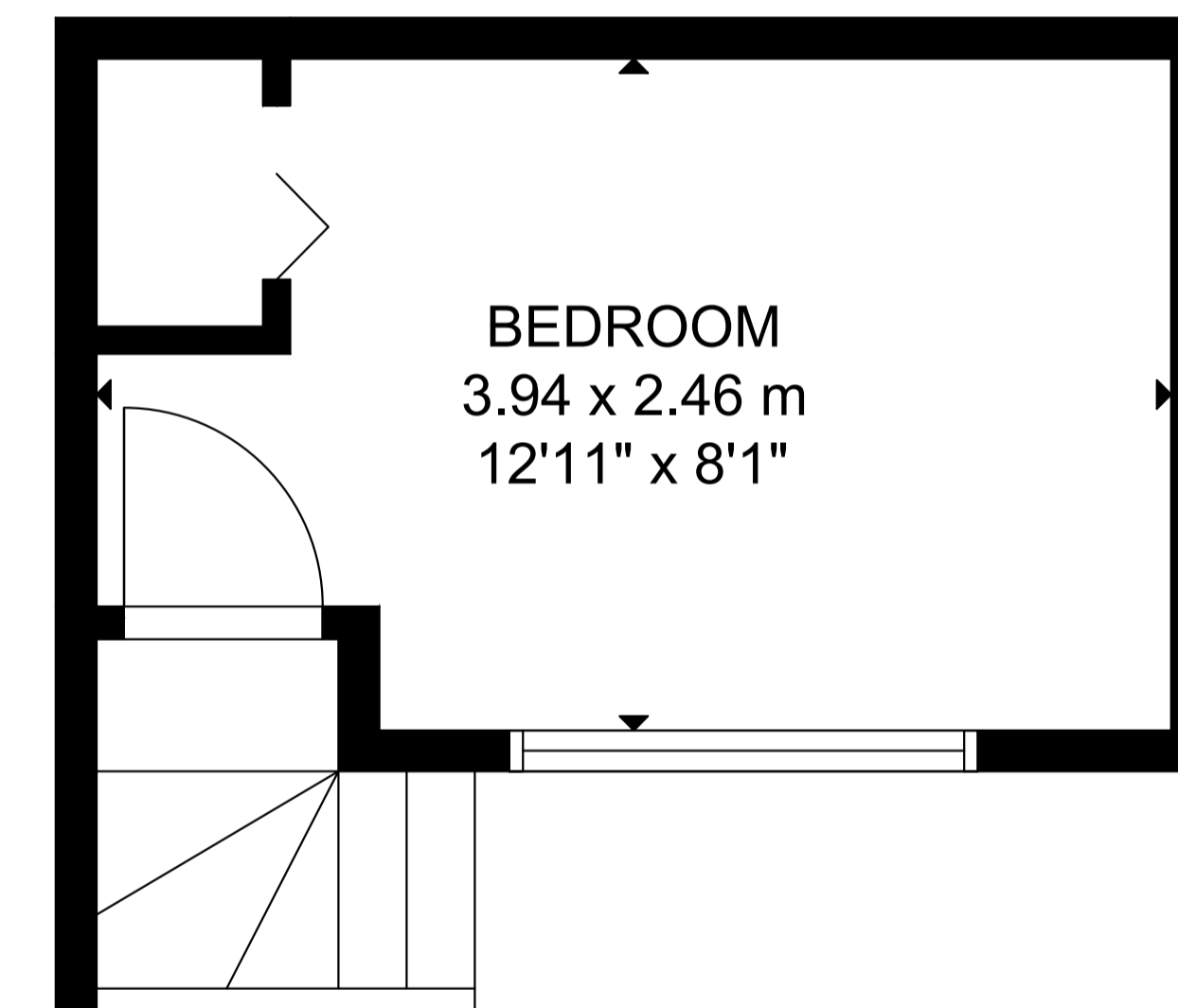
THIRD FLOOR
