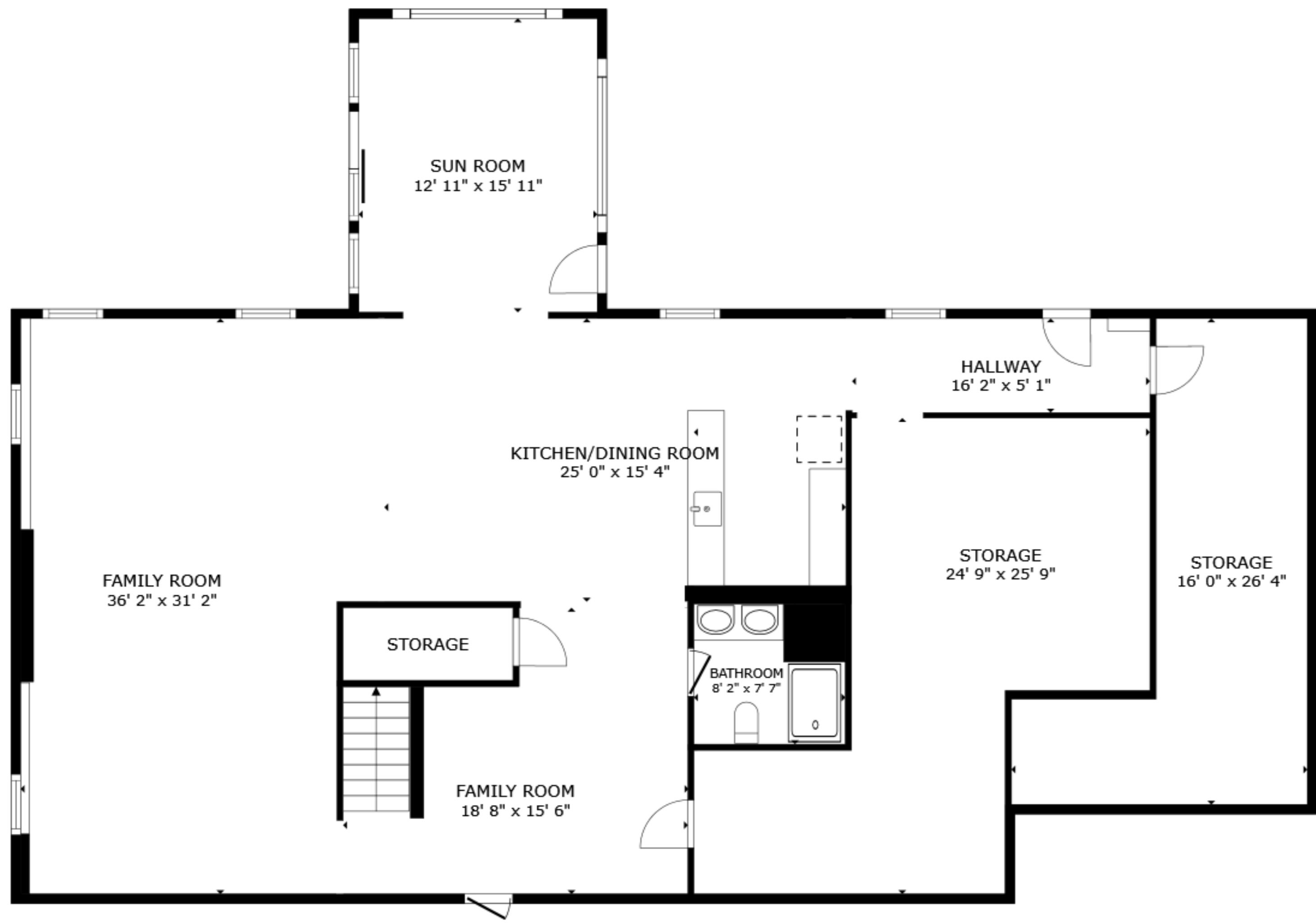
FLOOR 1
