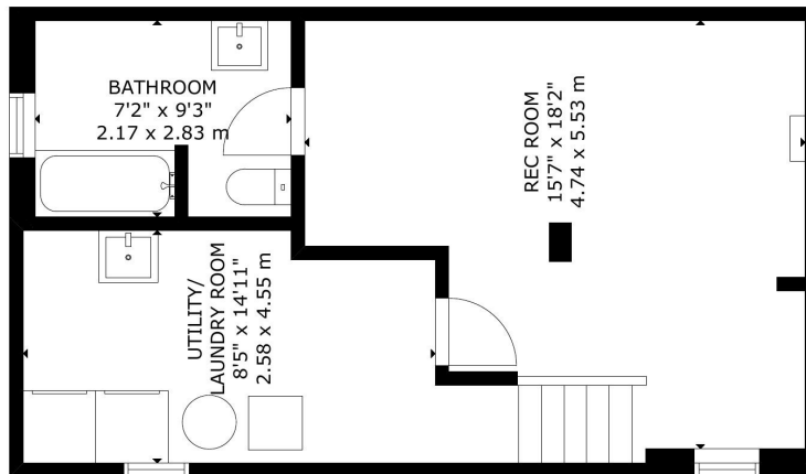
LOWER FLOOR
