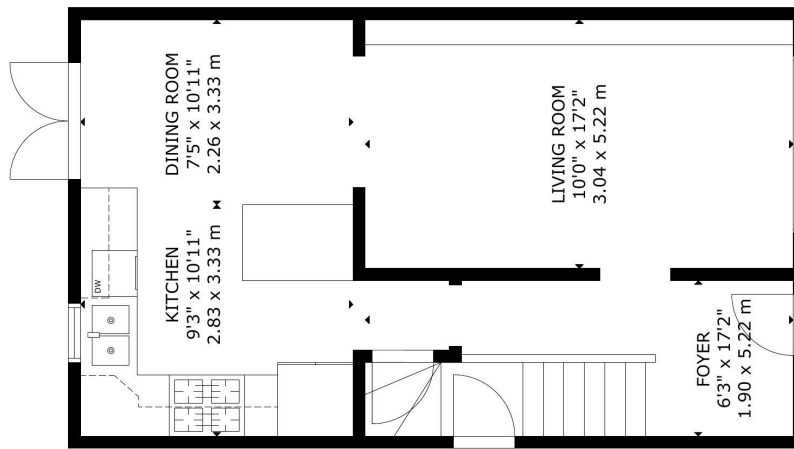
MAIN FLOOR
