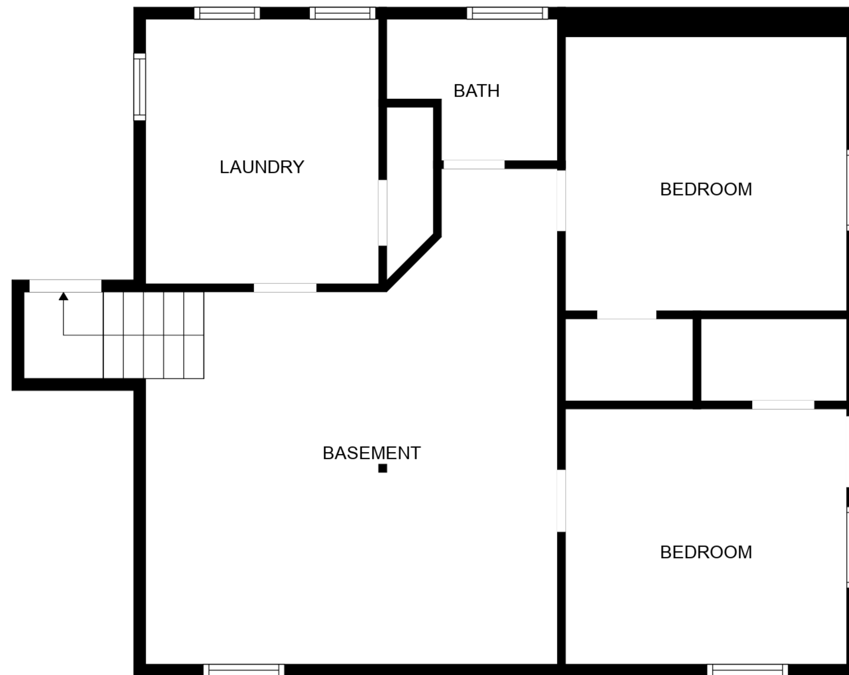
FLOOR 1
