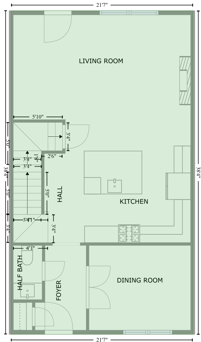
FLOOR 2 [AREA: 827]
