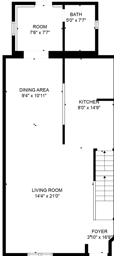
FLOOR 2
