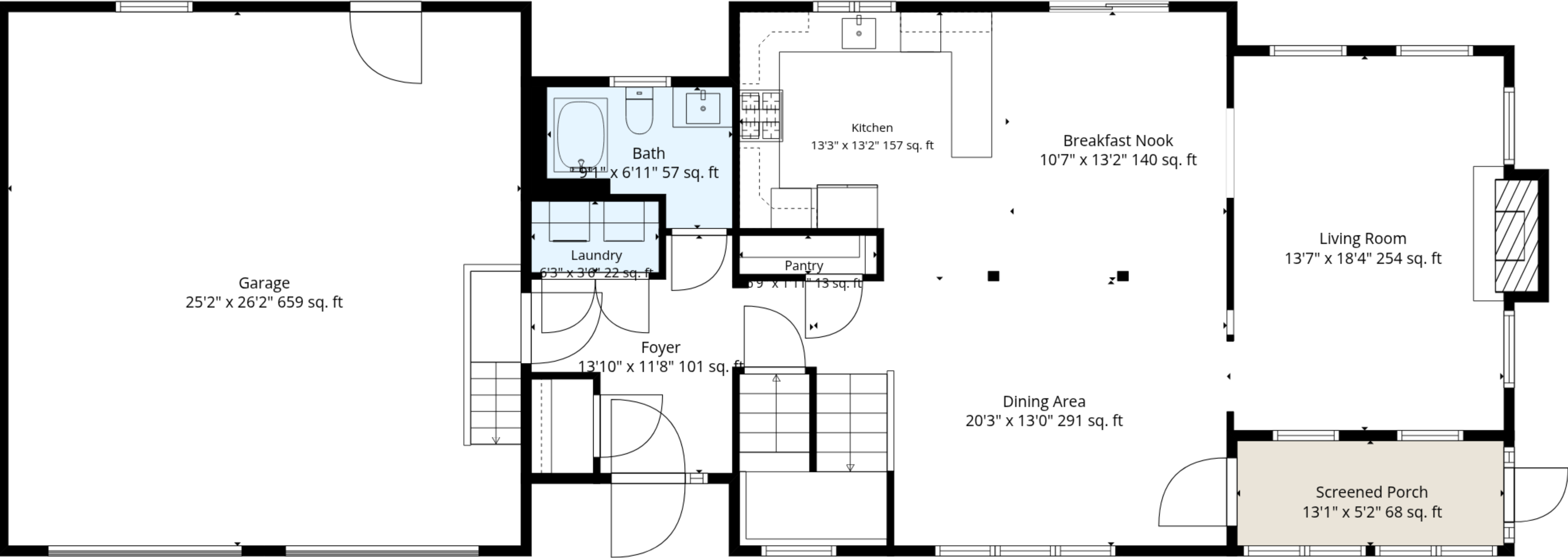
1st Floor
