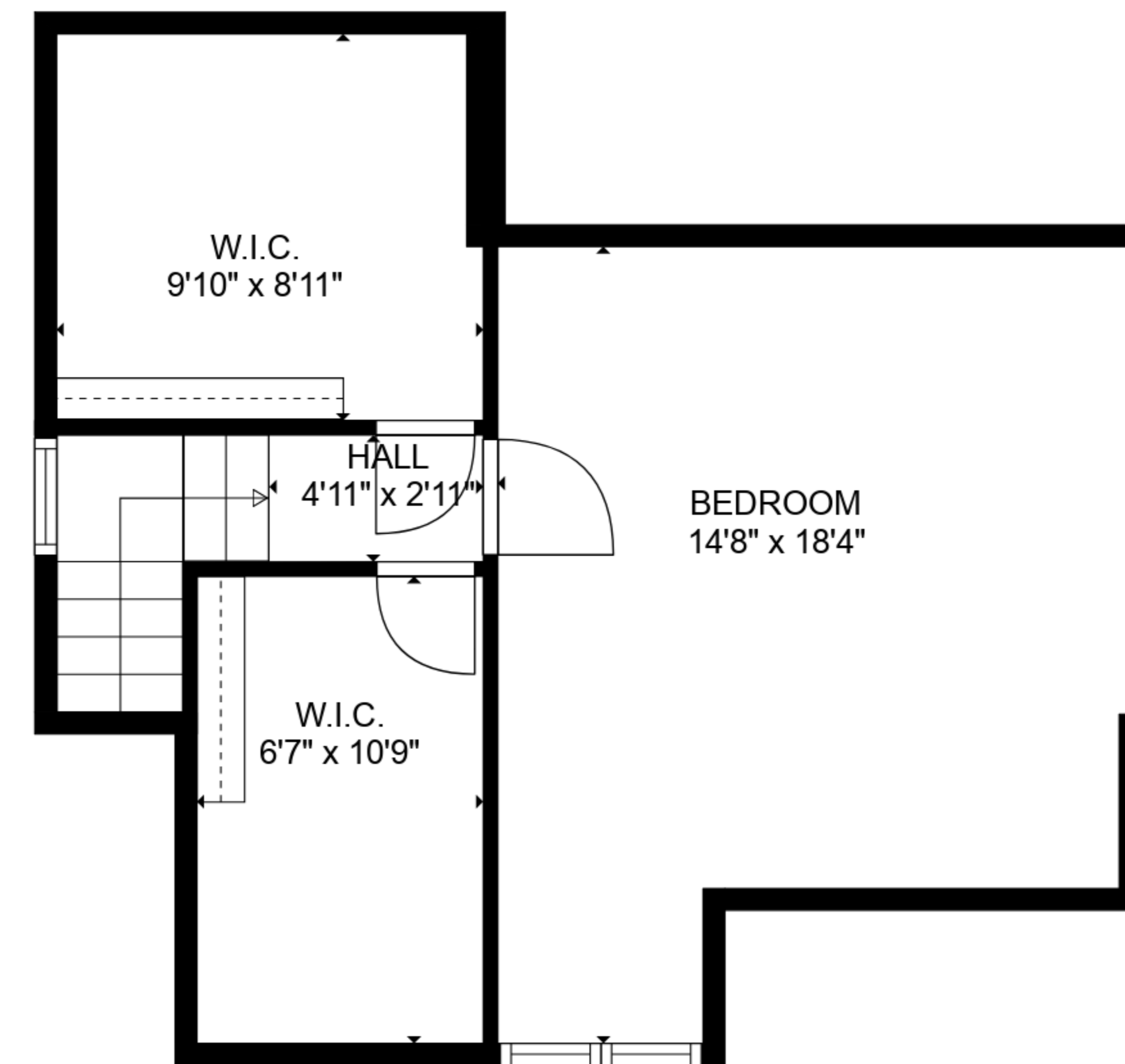
FLOOR 4
