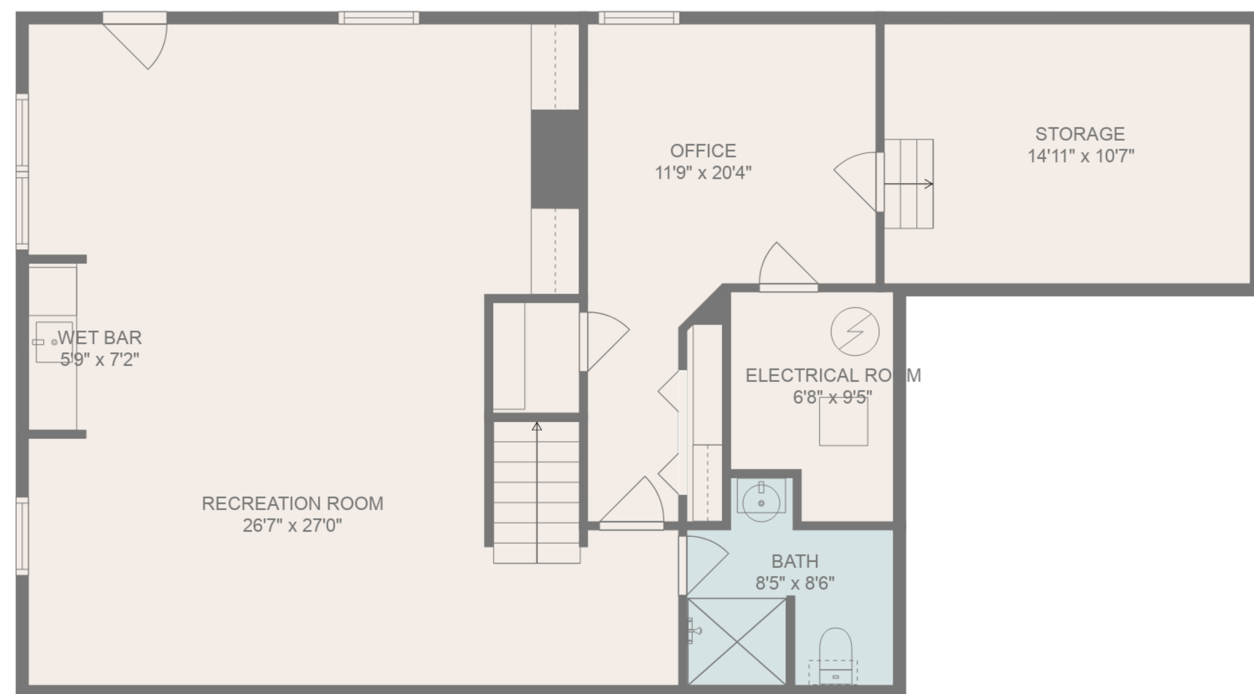
FLOOR 1
