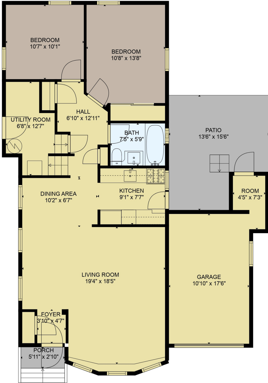
FLOOR 1
