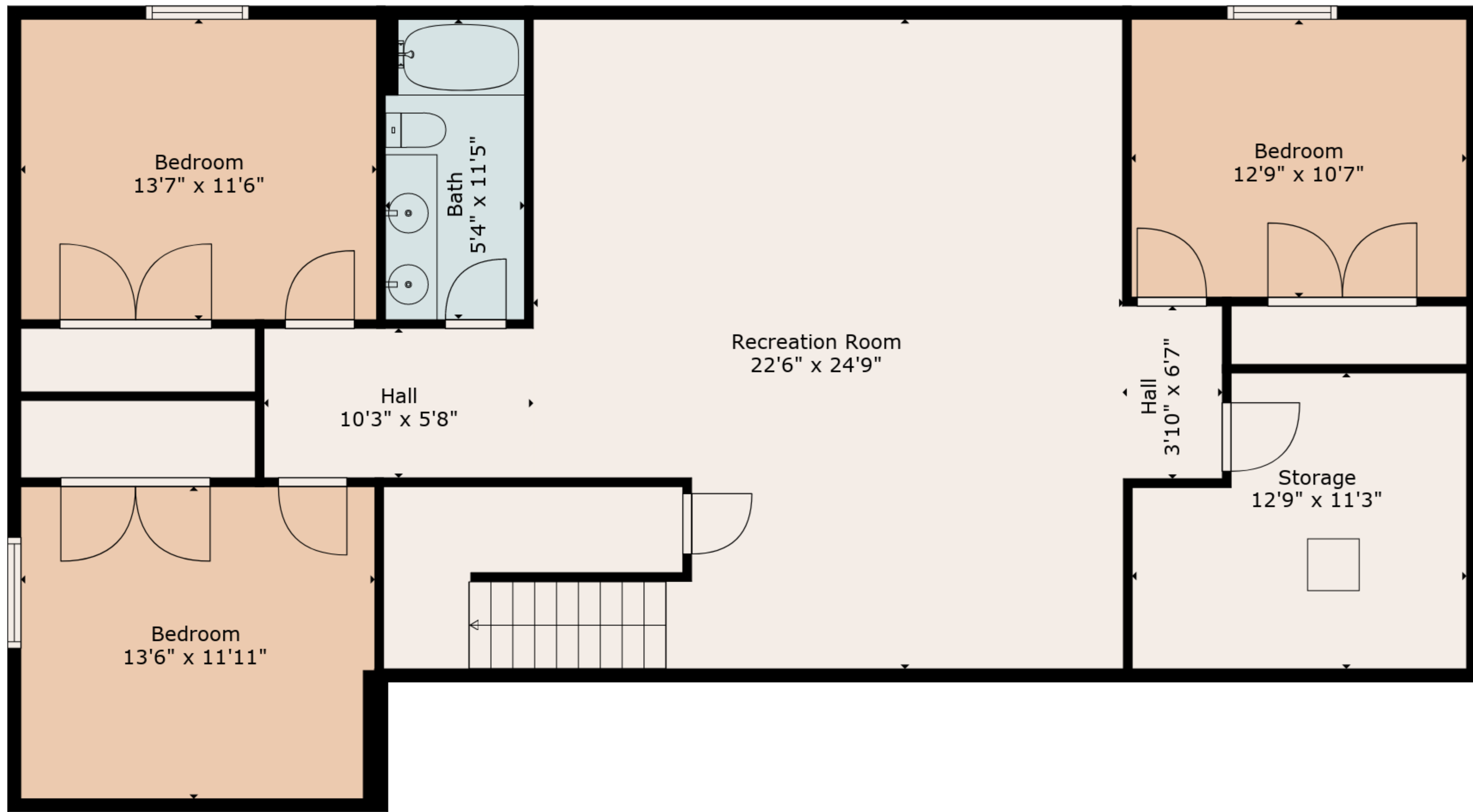
Floor 1
