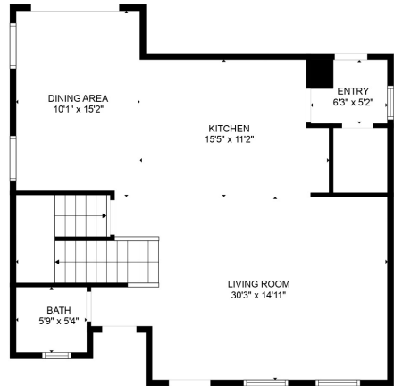
FLOOR 2
