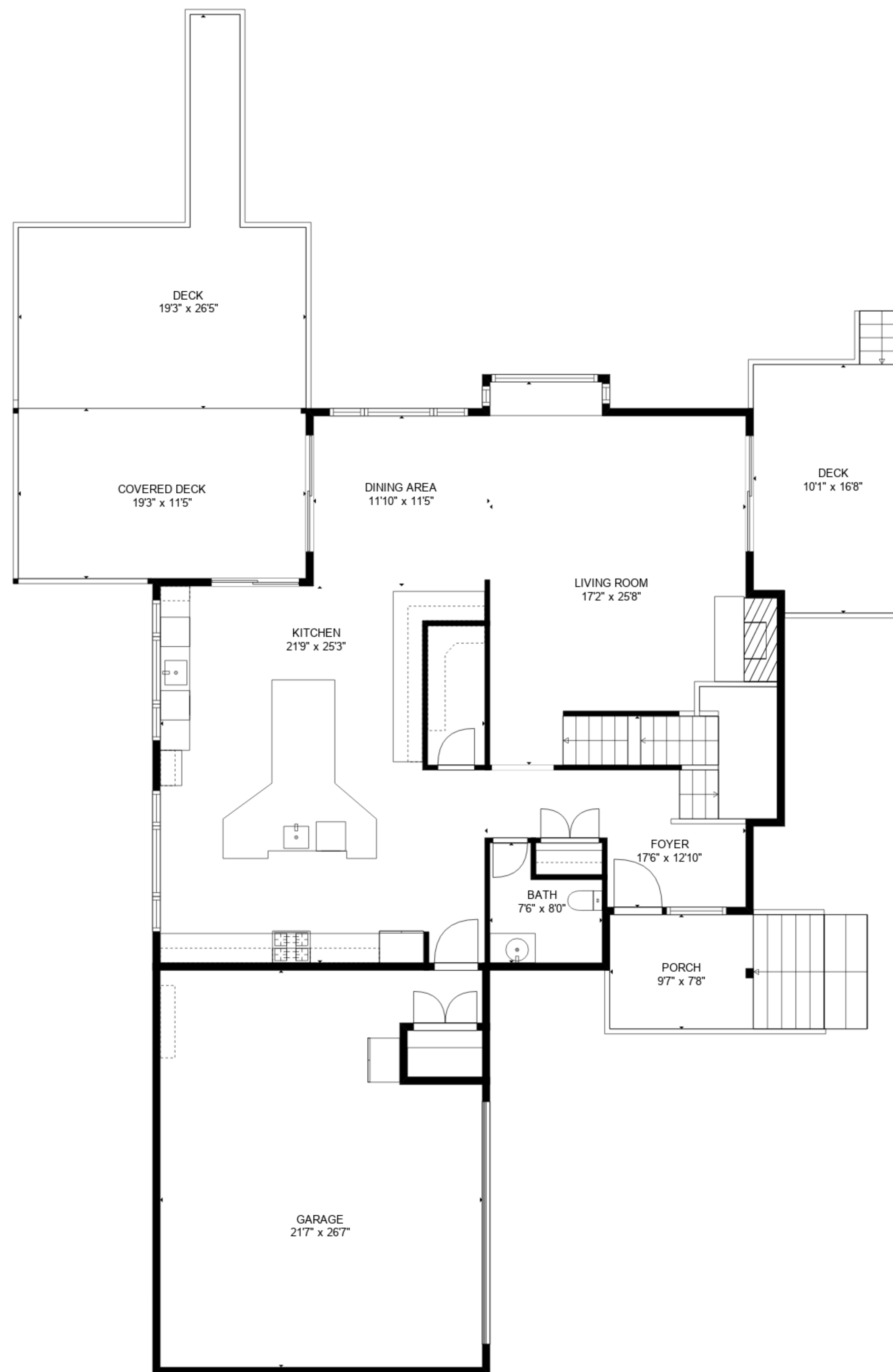
FLOOR 2
