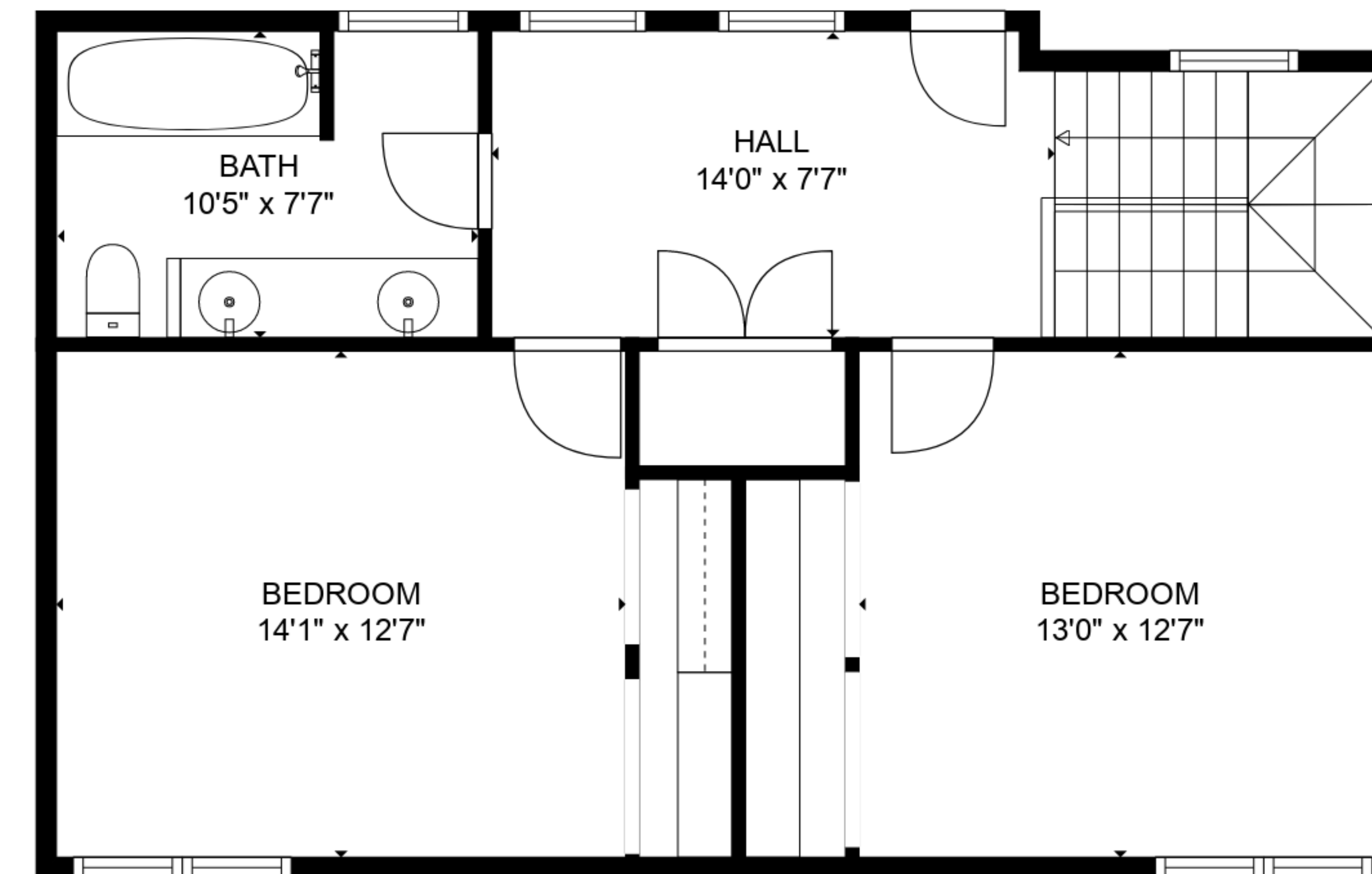
FLOOR 2
