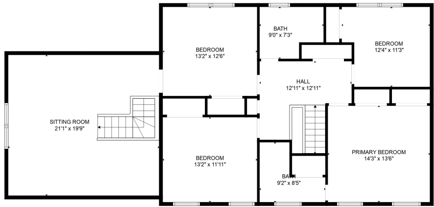
FLOOR 2
