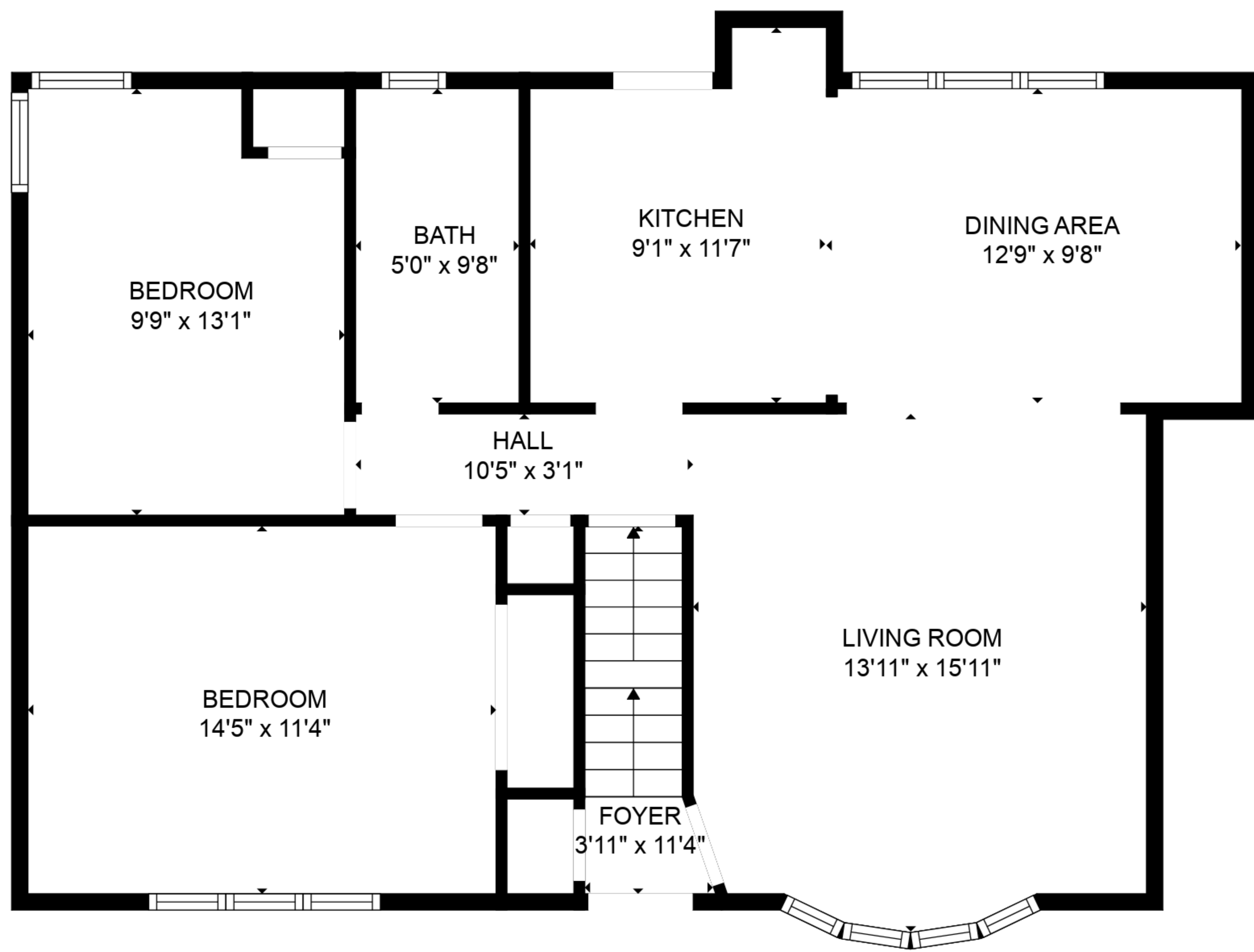
FLOOR 2
