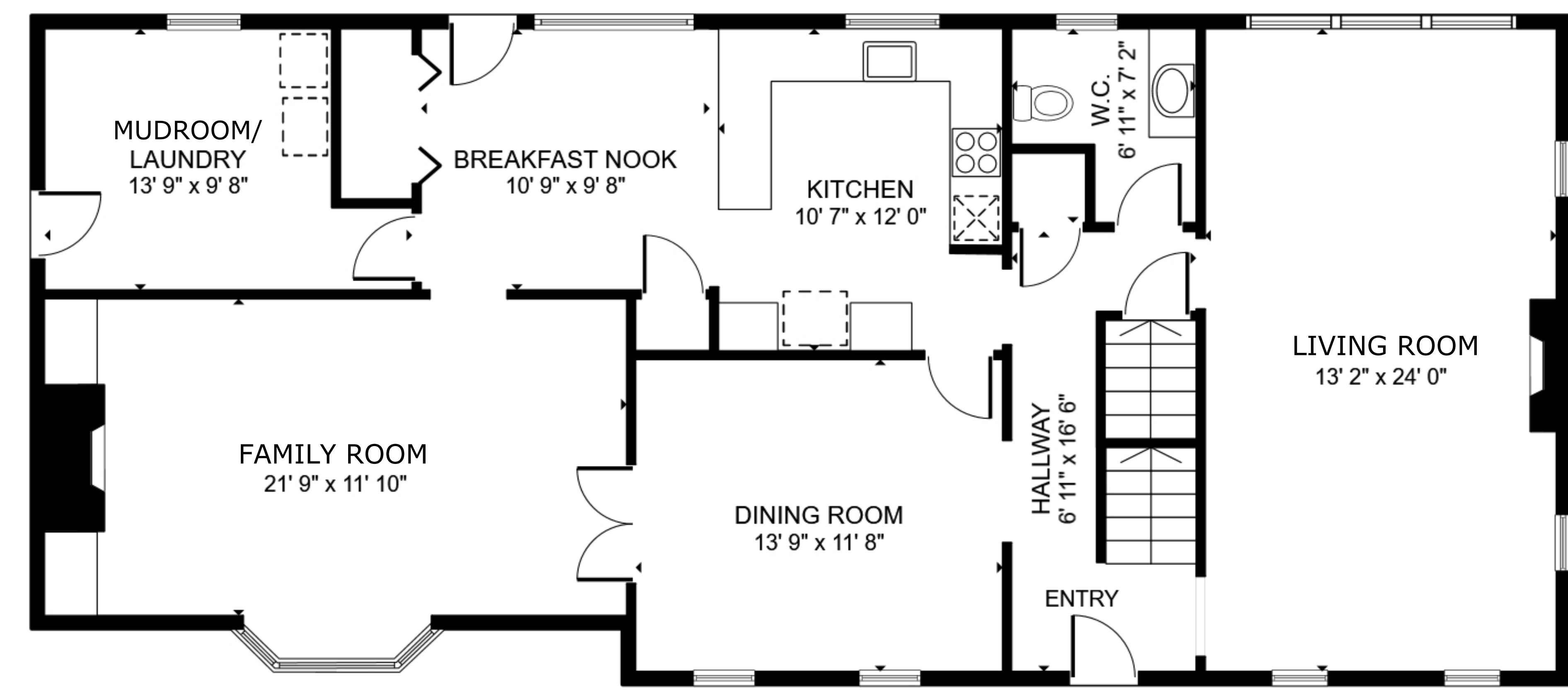
FLOOR 2
