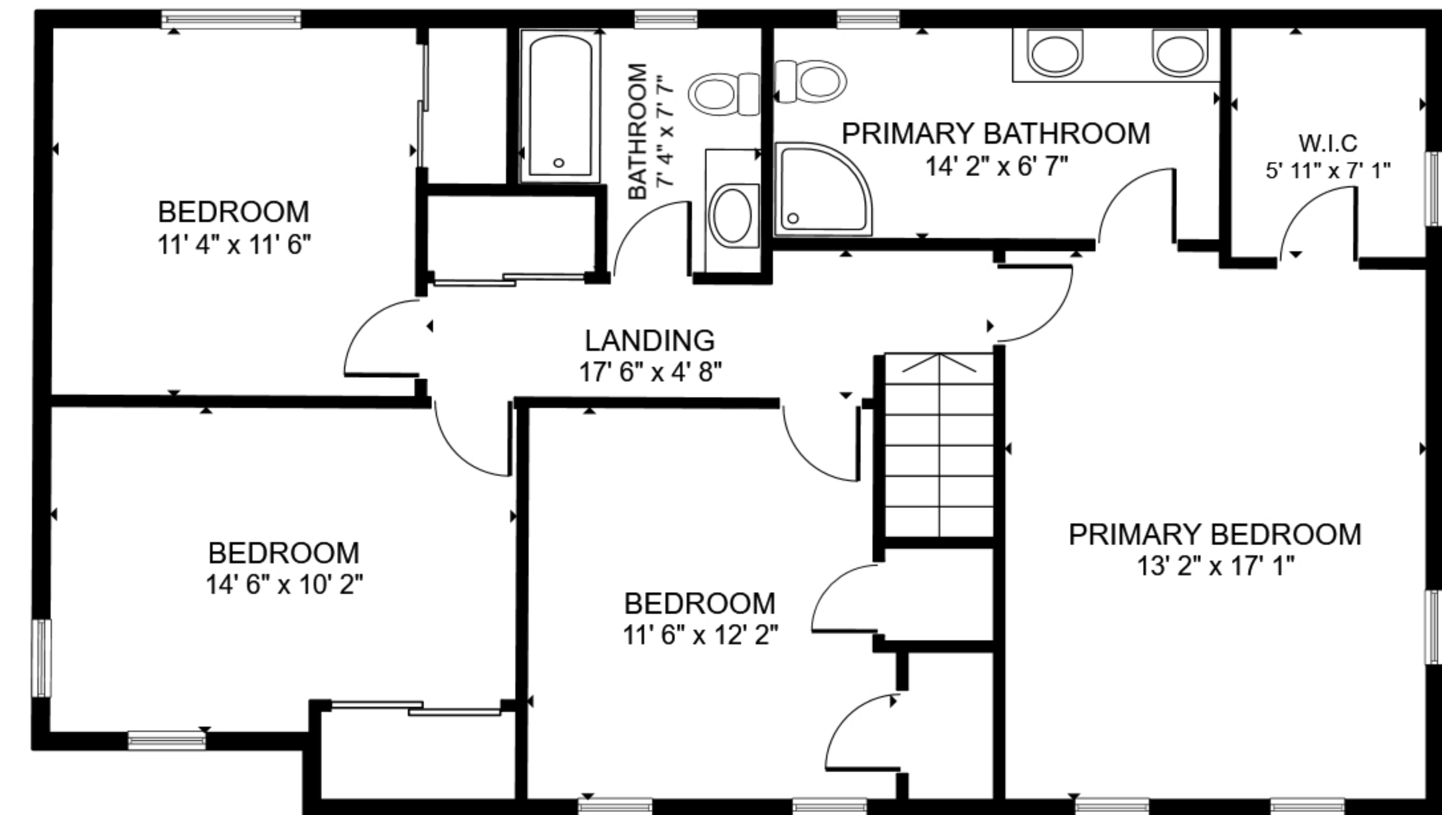
FLOOR 3
