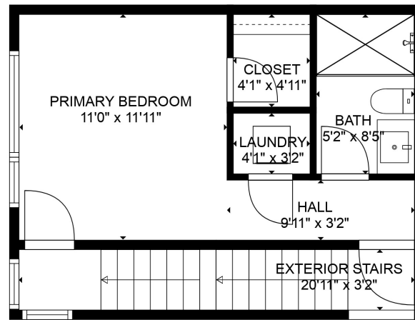
UPPER LEVEL
