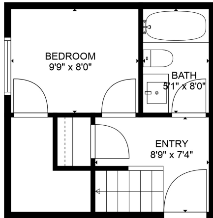
LOWER LEVEL
