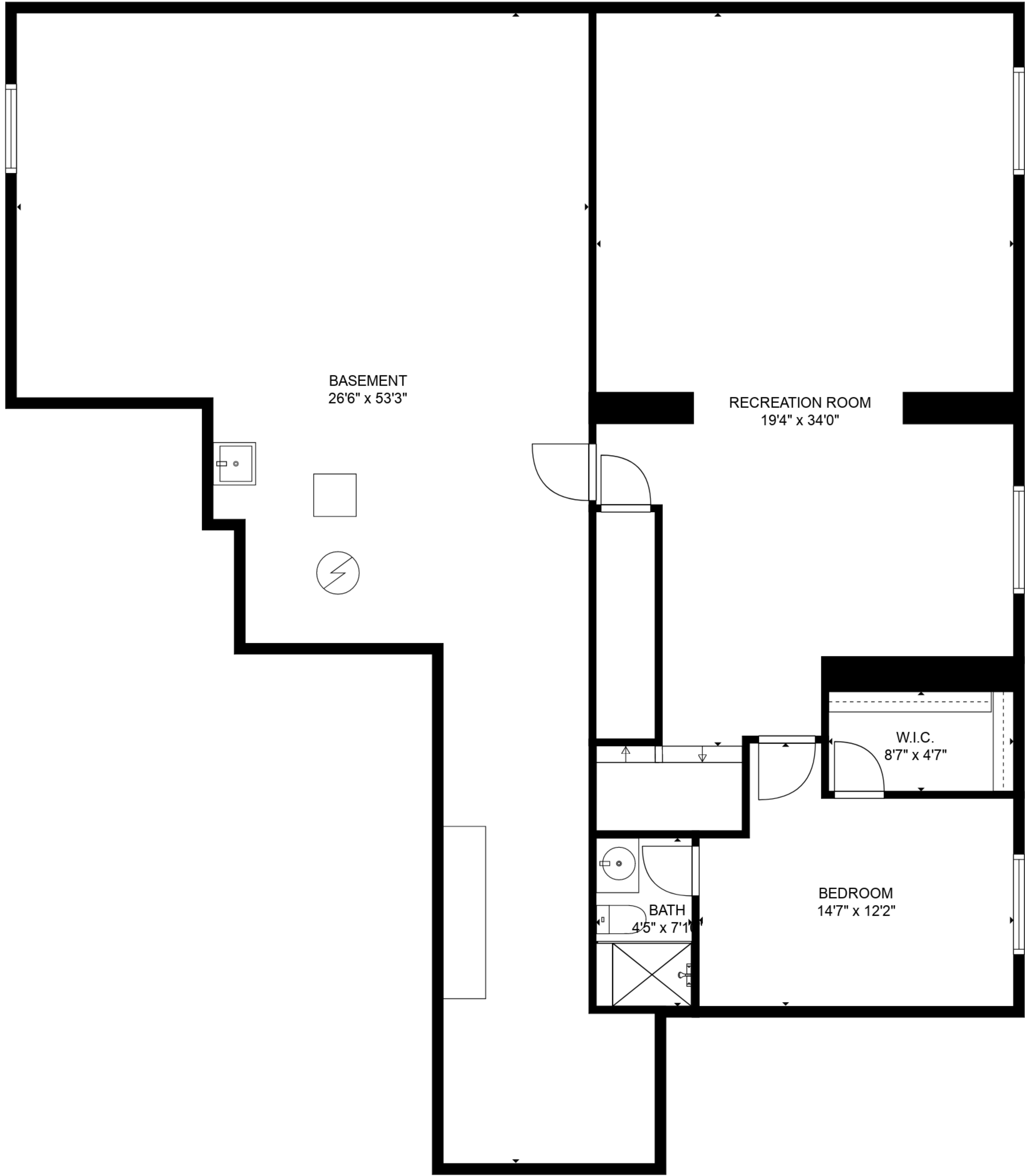
FLOOR 1
