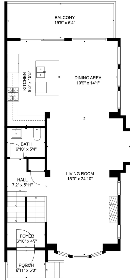
MAIN LEVEL
