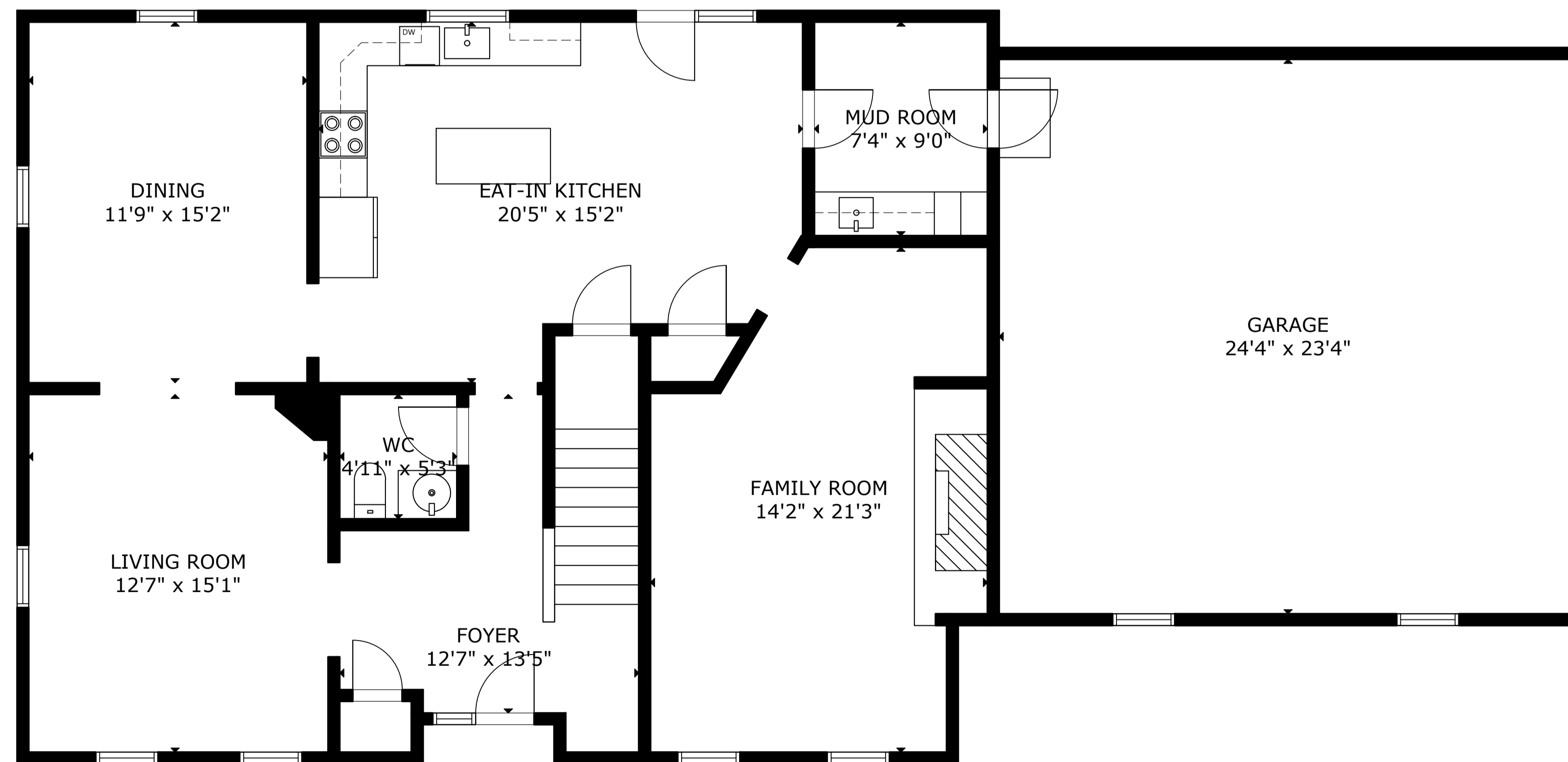
FIRST FLOOR
