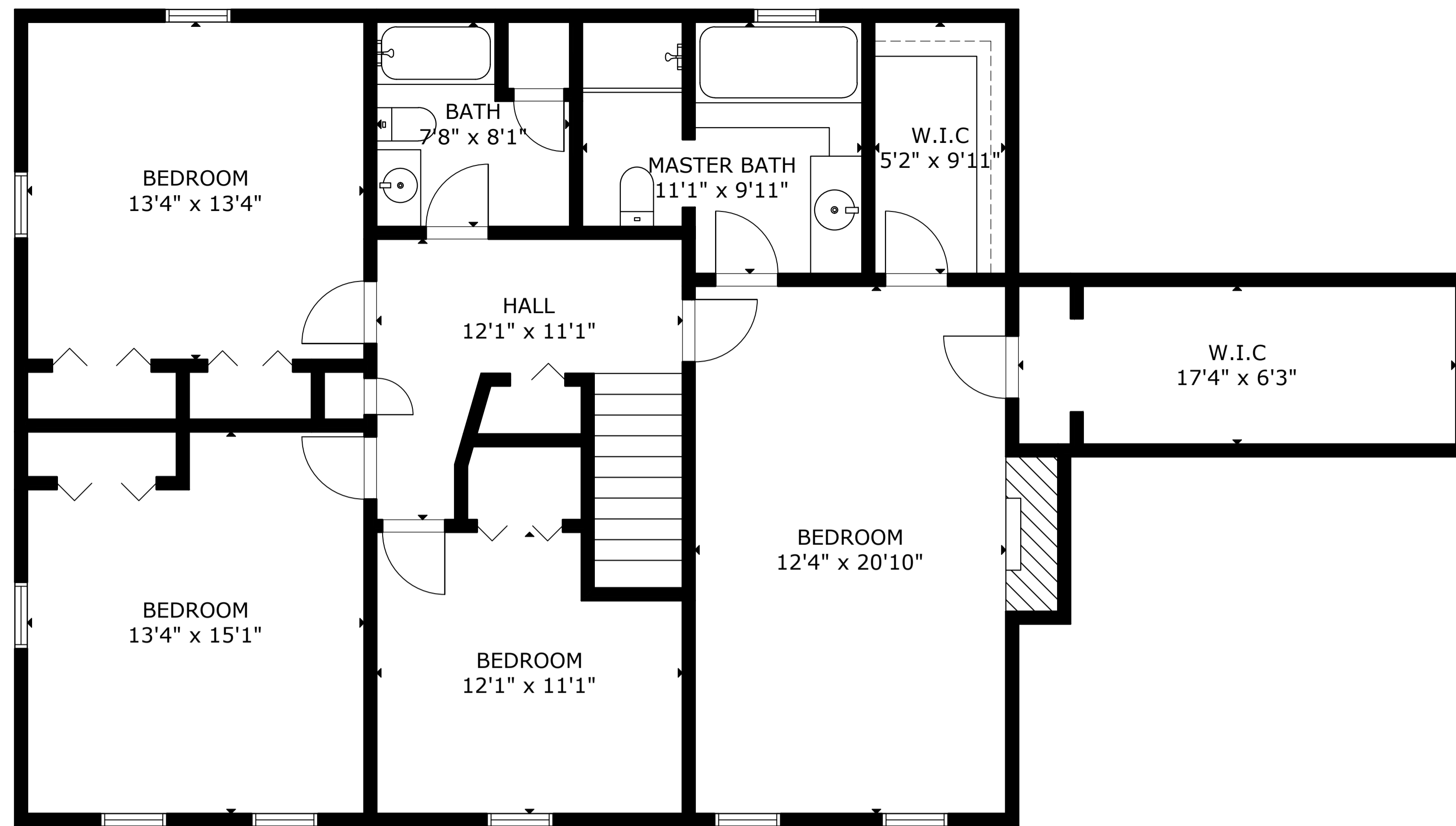
SECOND FLOOR
