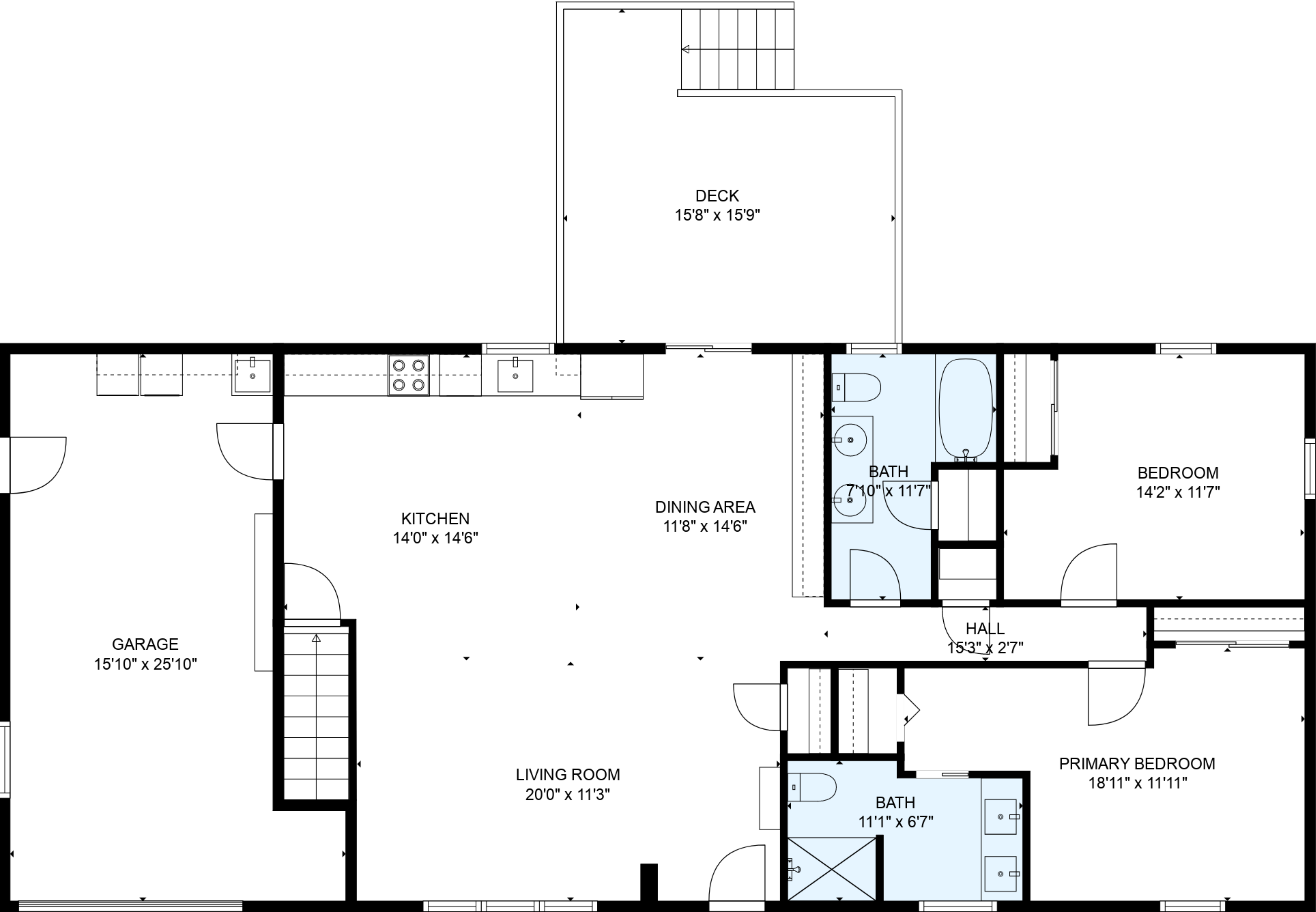
FLOOR 2
