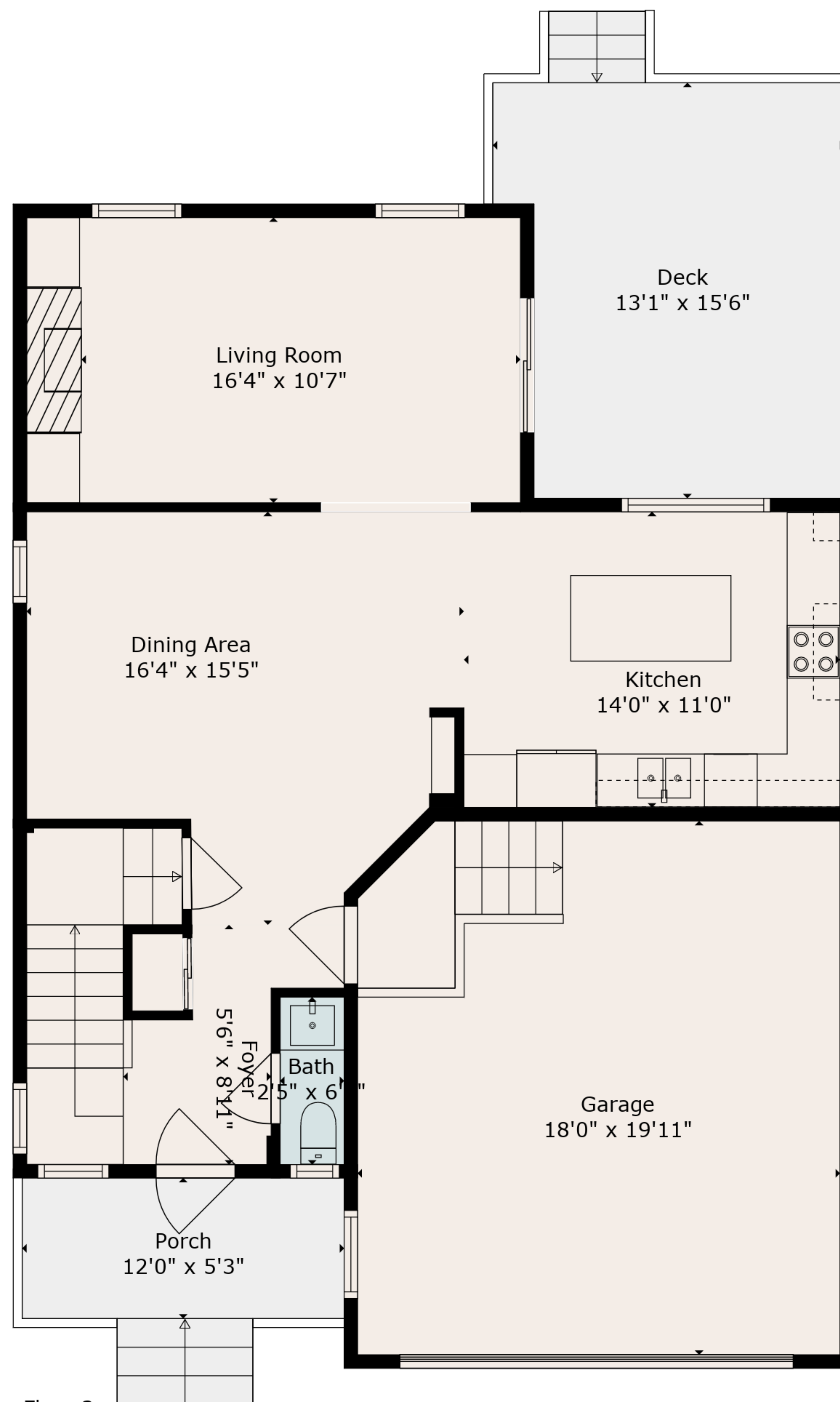
Floor 2
