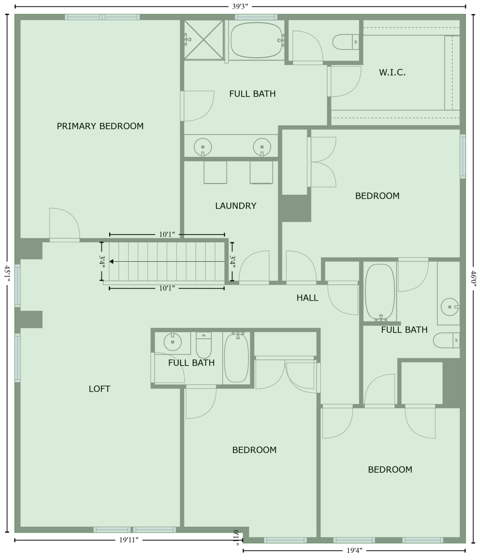
FLOOR 2 [AREA: 1788]
