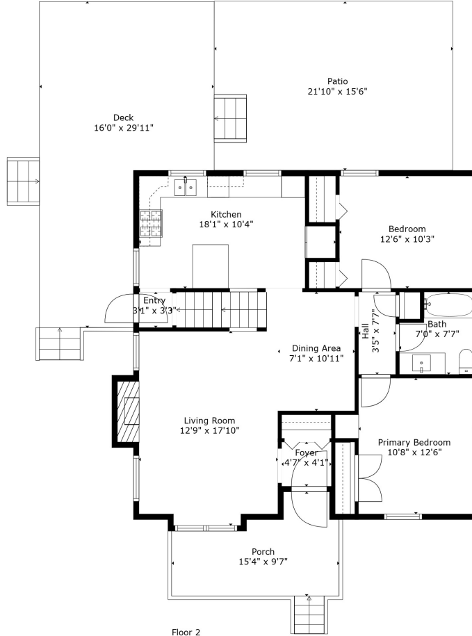
Floor 2
