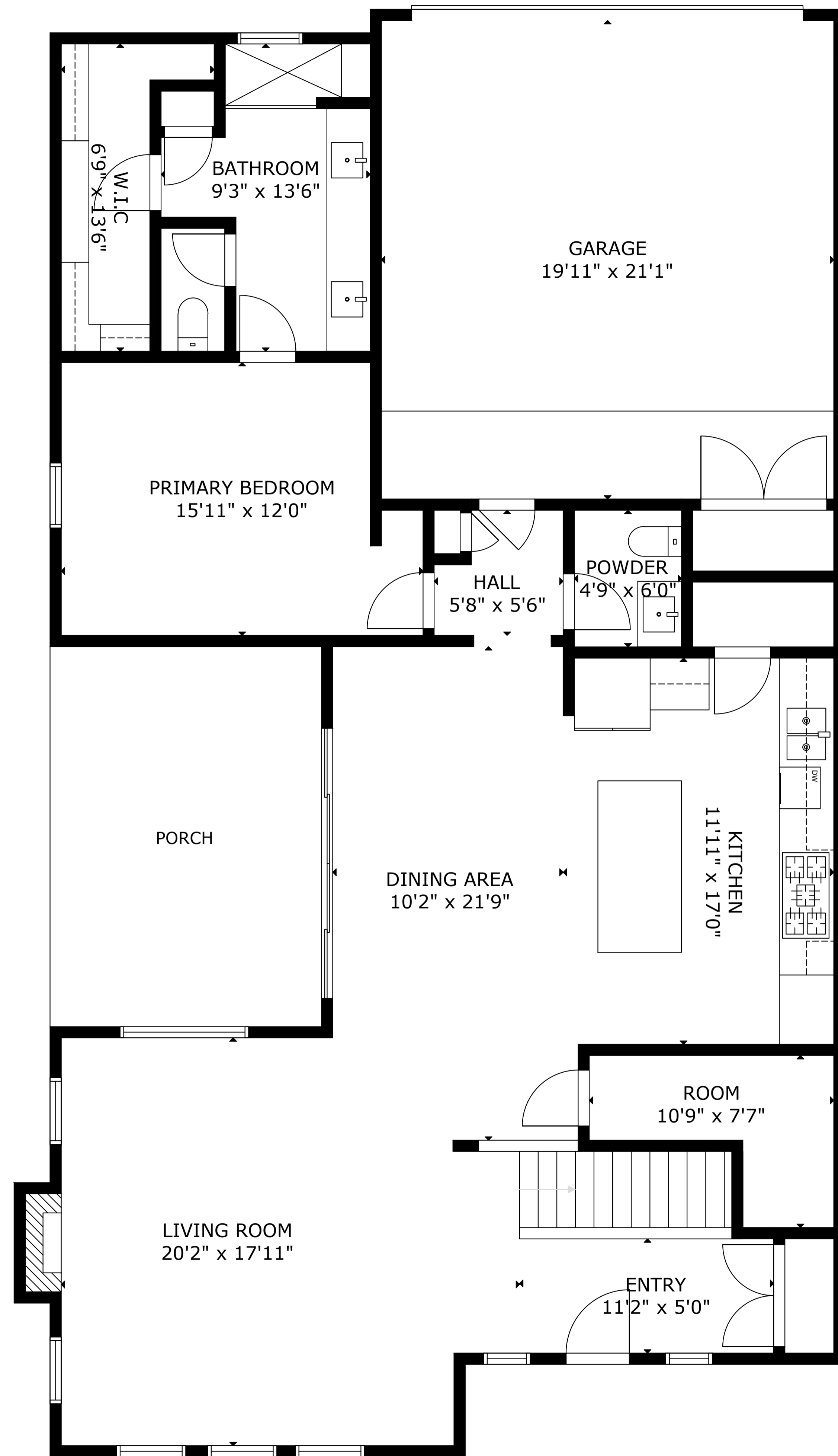
FLOOR 1
