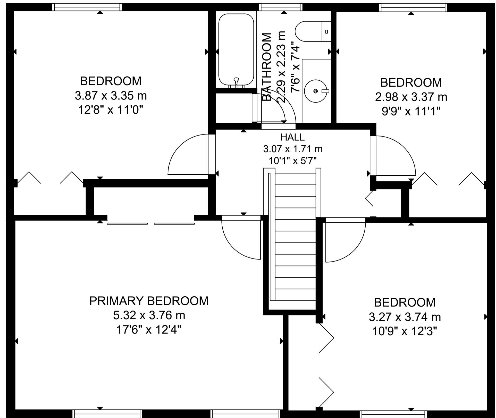
SECOND FLOOR
