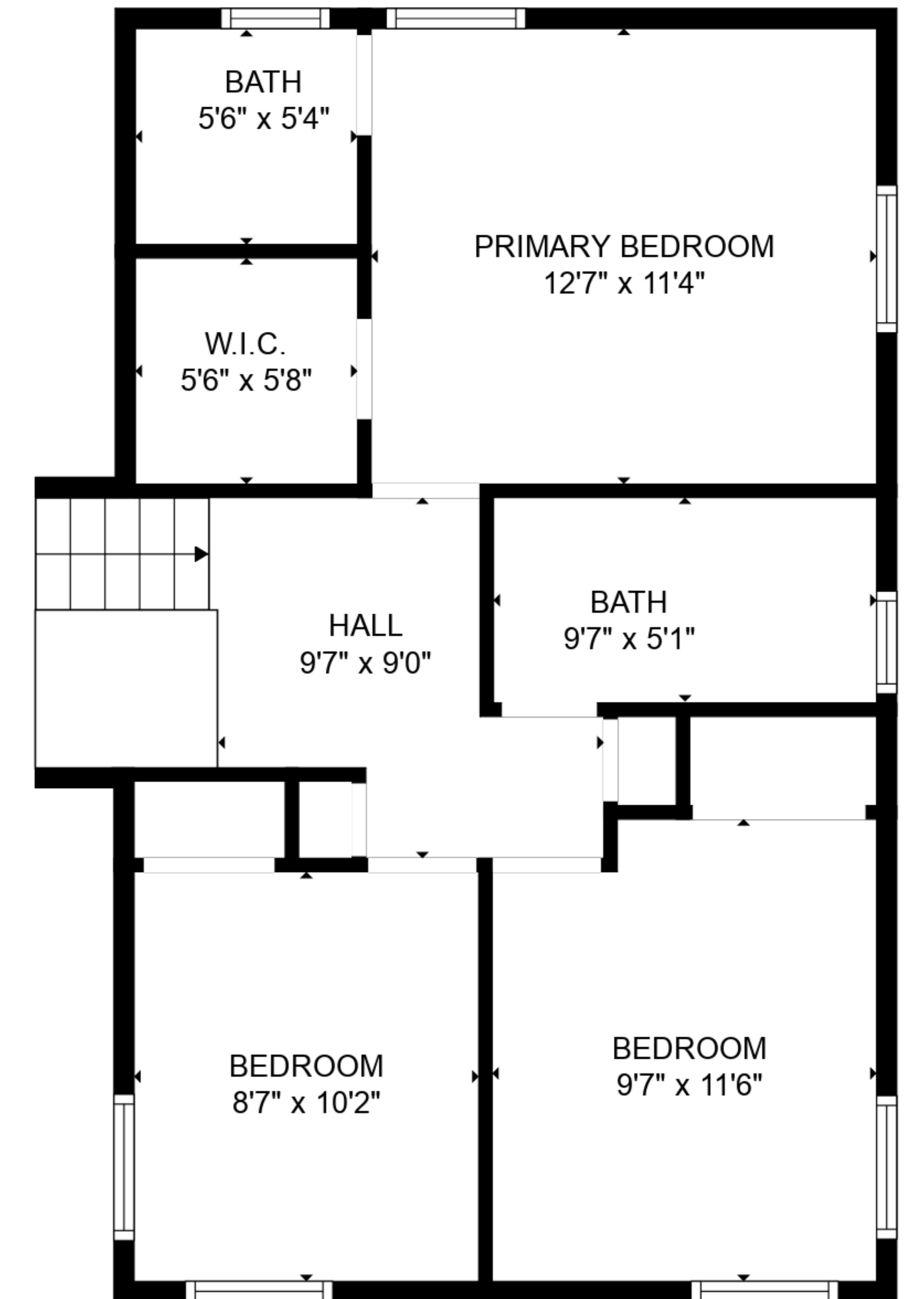
FLOOR 4
