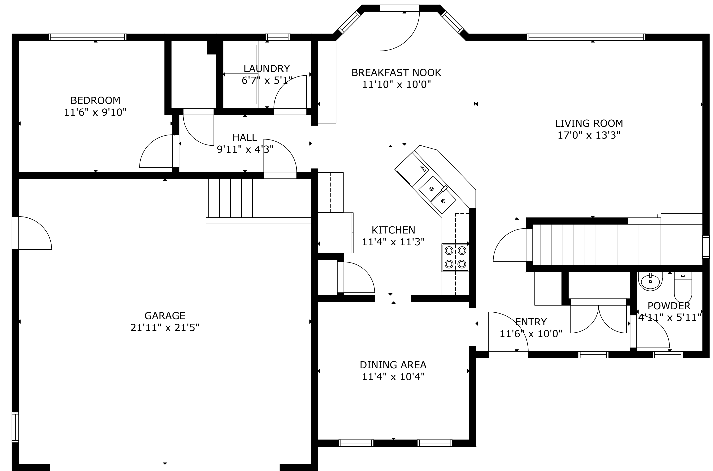
MAIN FLOOR
