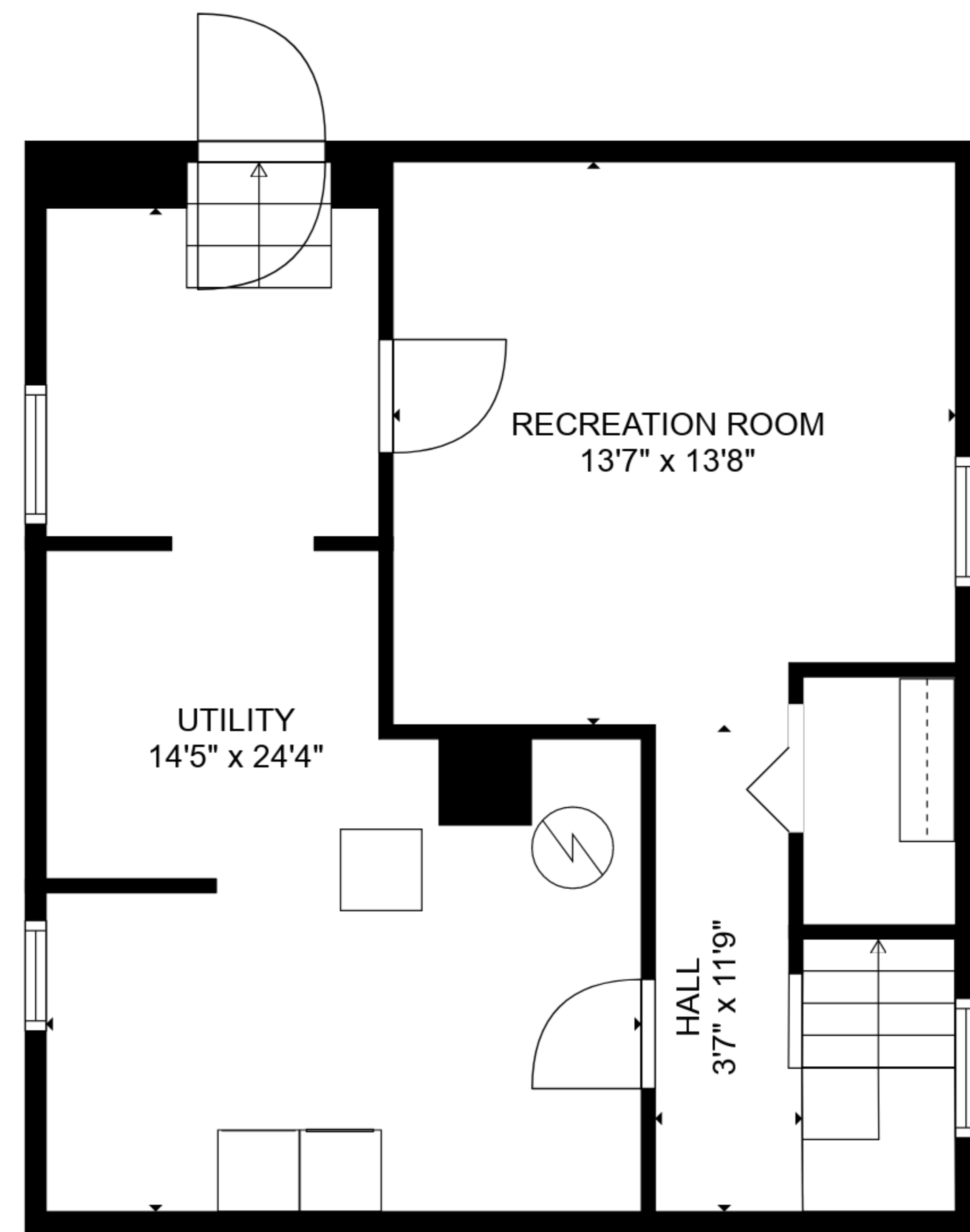
FLOOR 1
