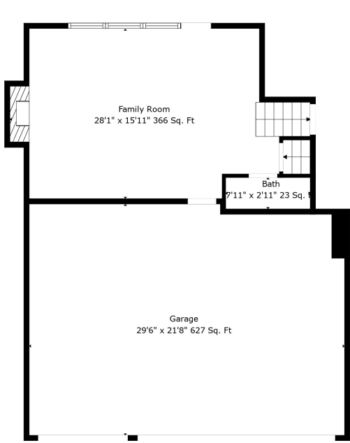
Floor 2
