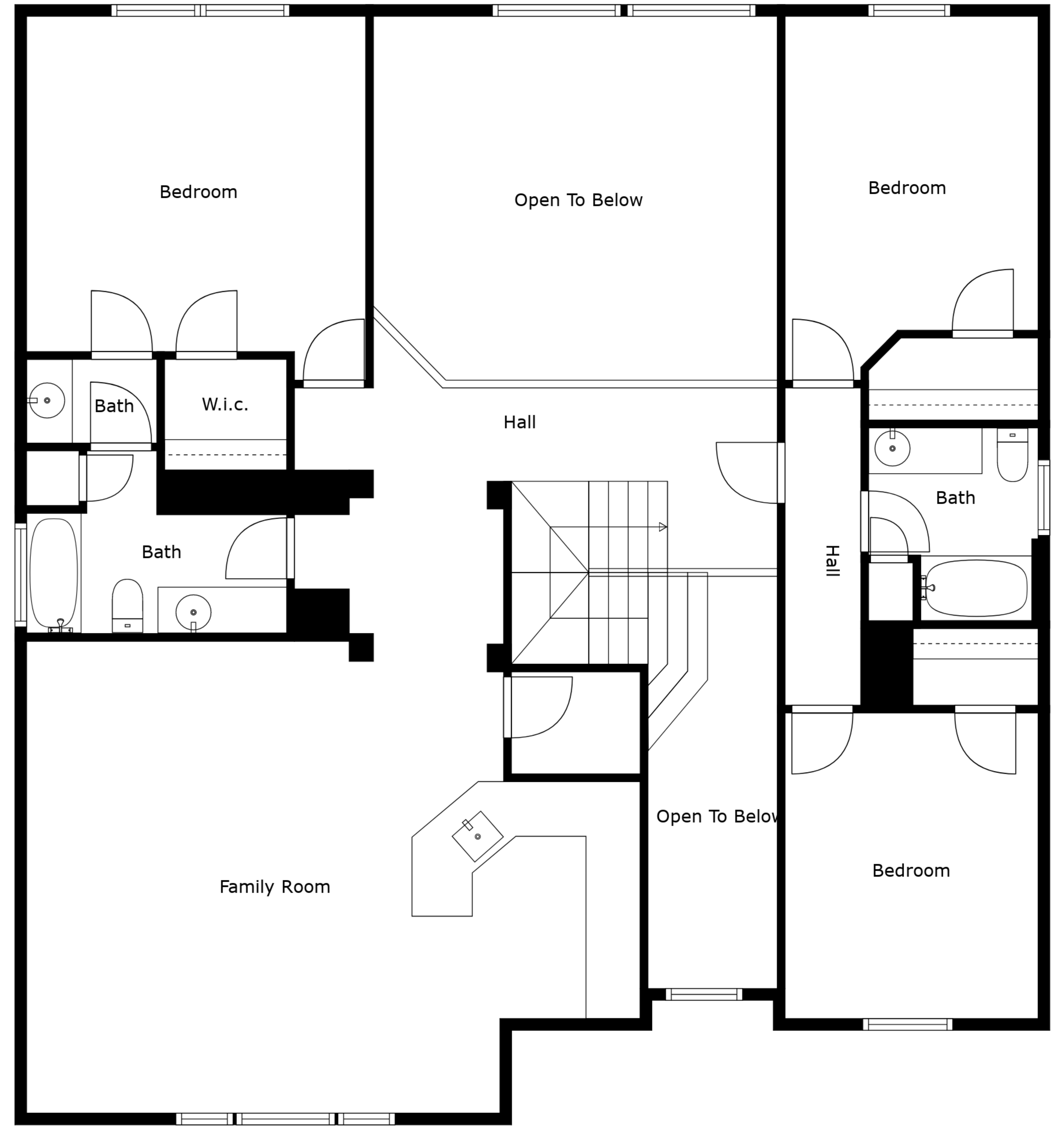
Floor 2
