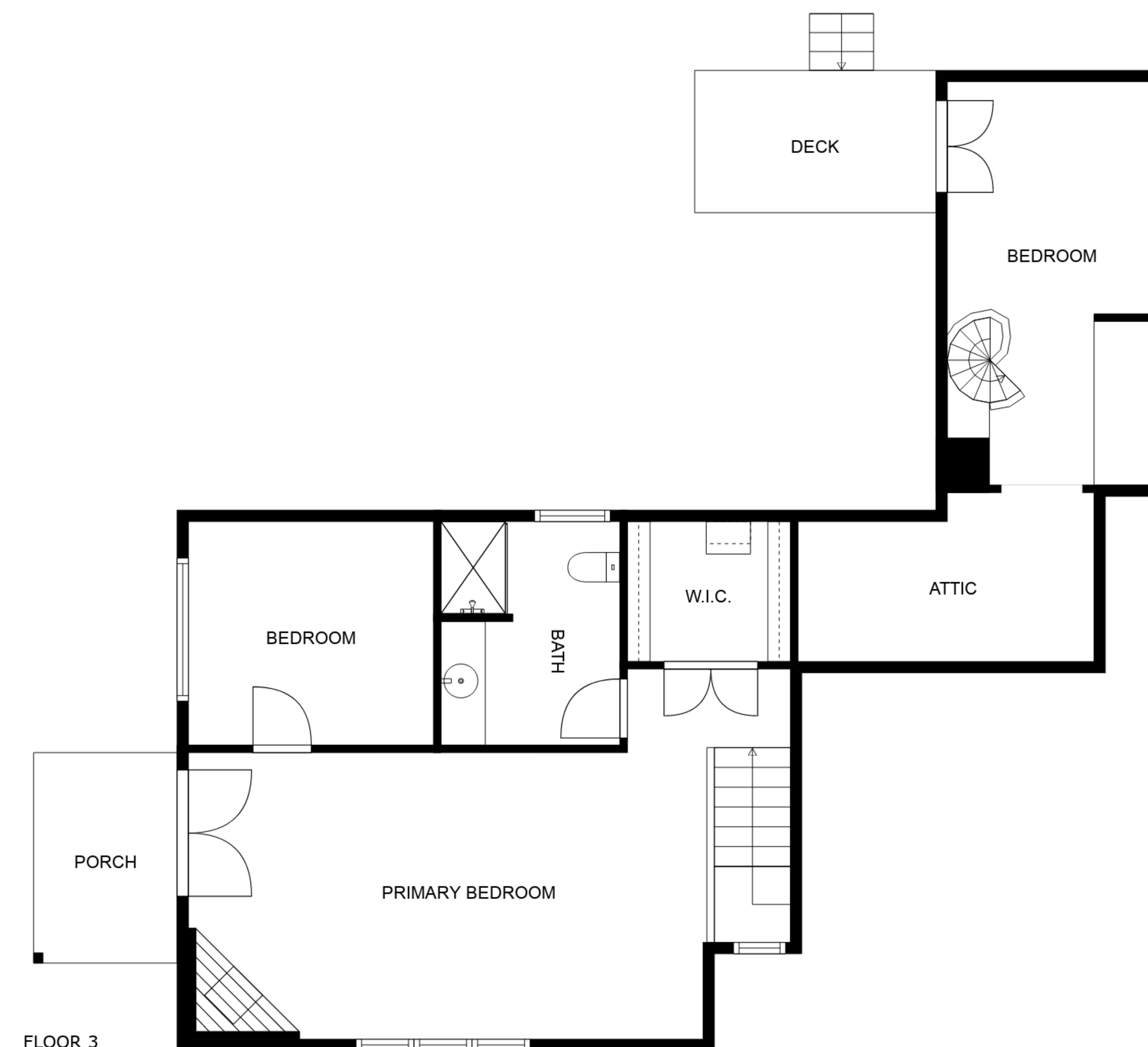
FLOOR 3
