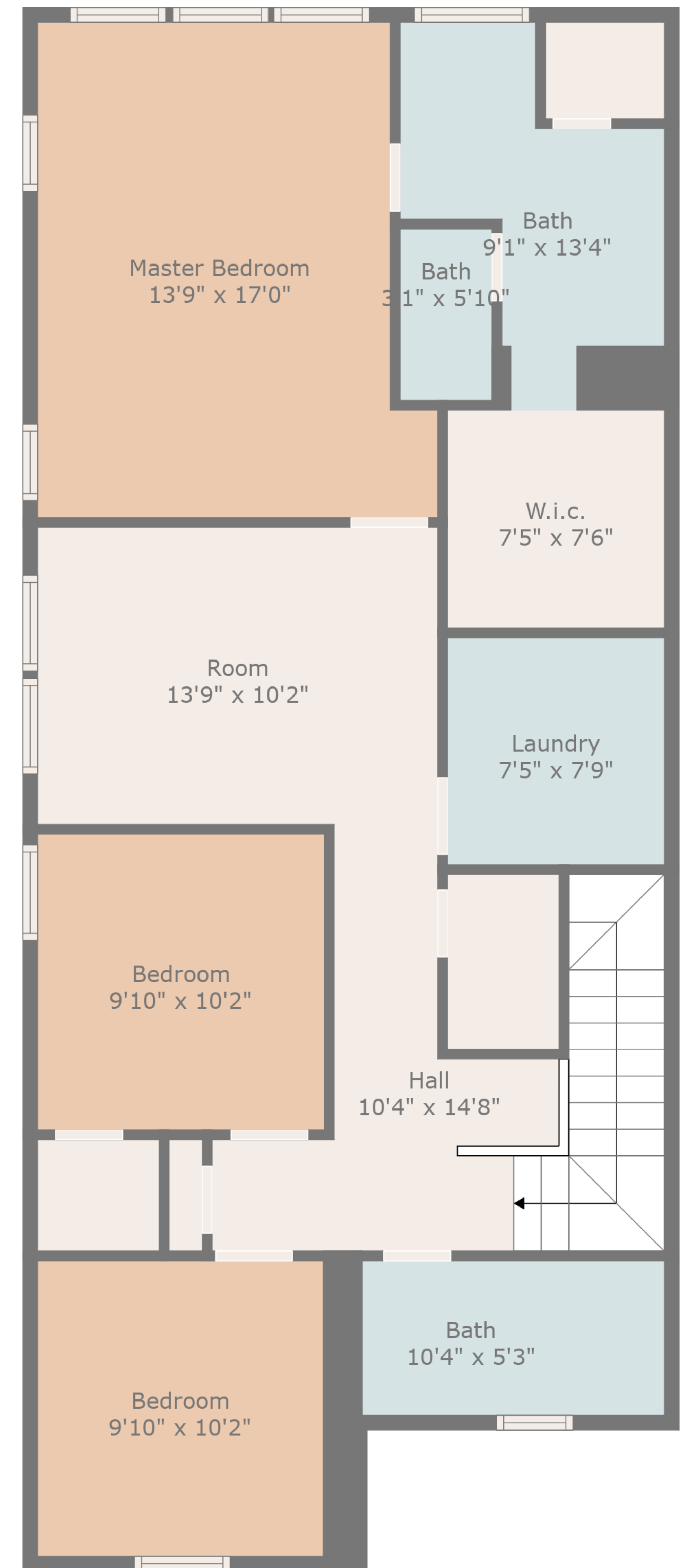
Floor 3
