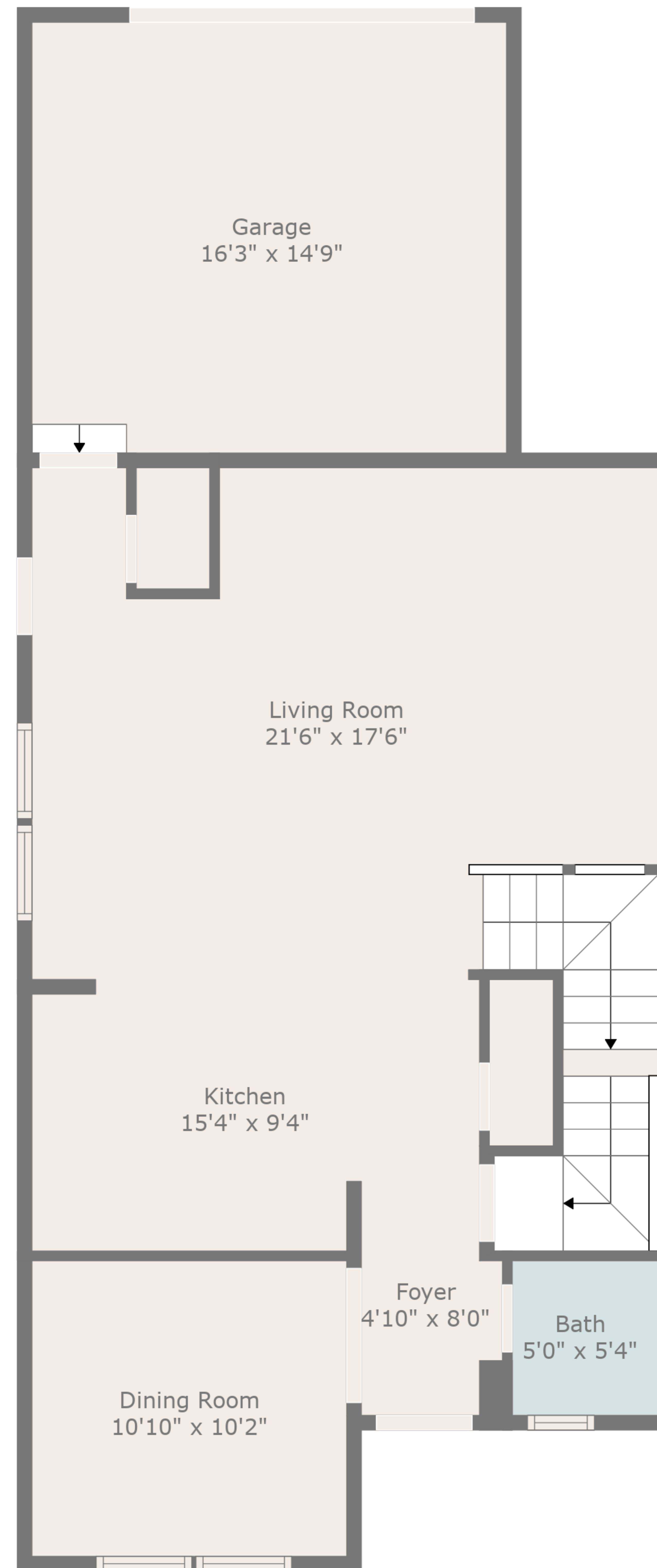
Floor 2
