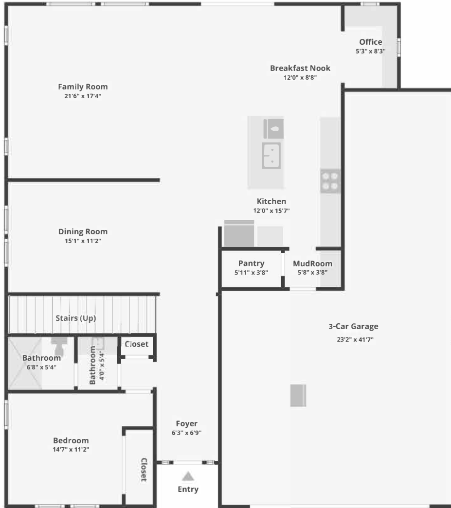
FLOOR 1
