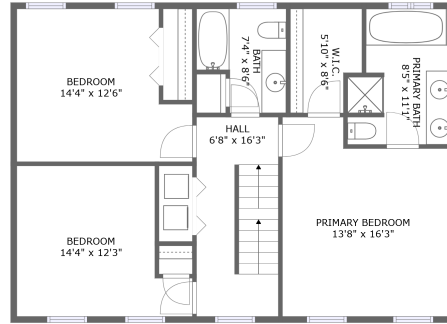
FLOOR 3
