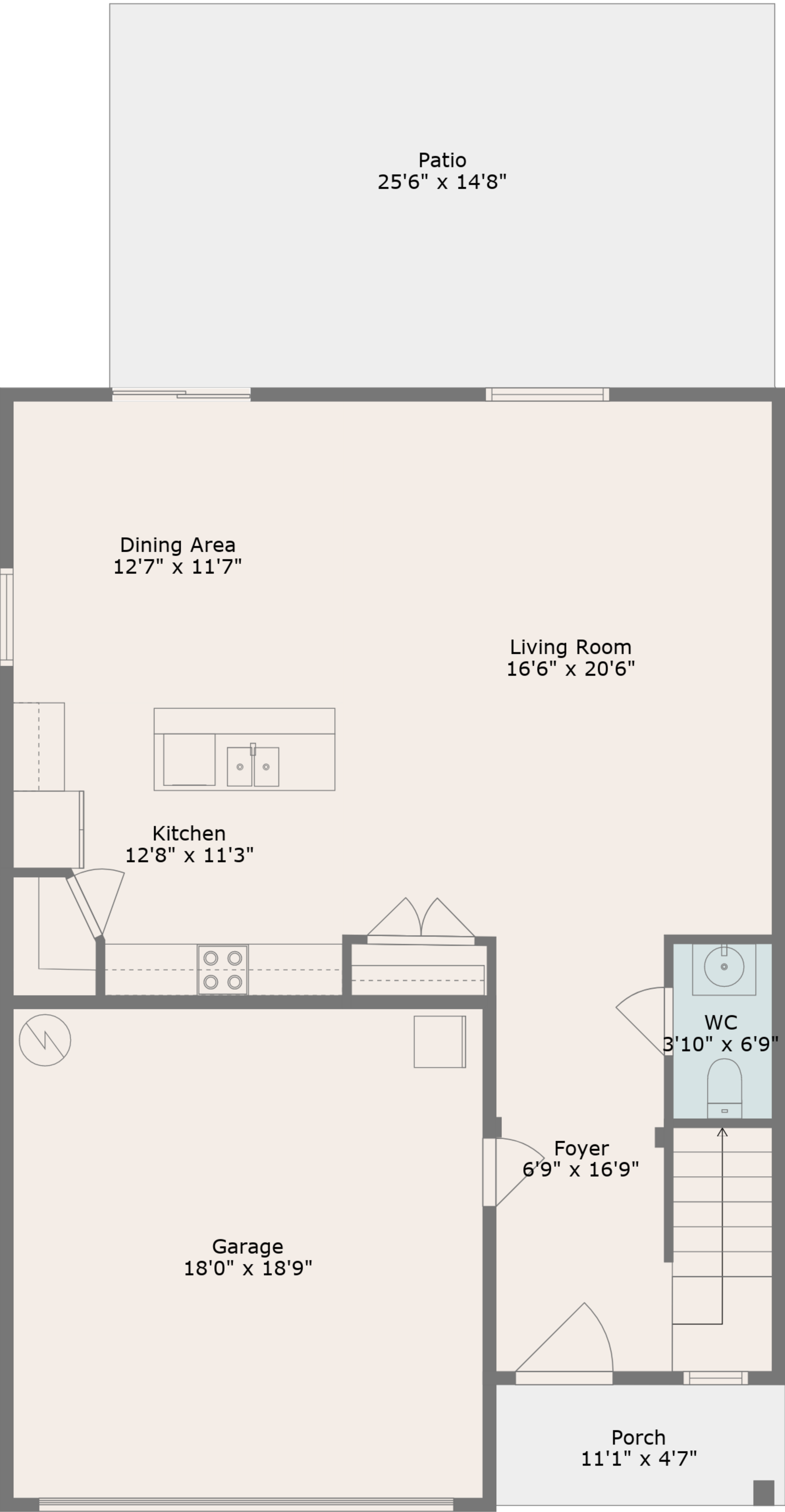
Floor 1
