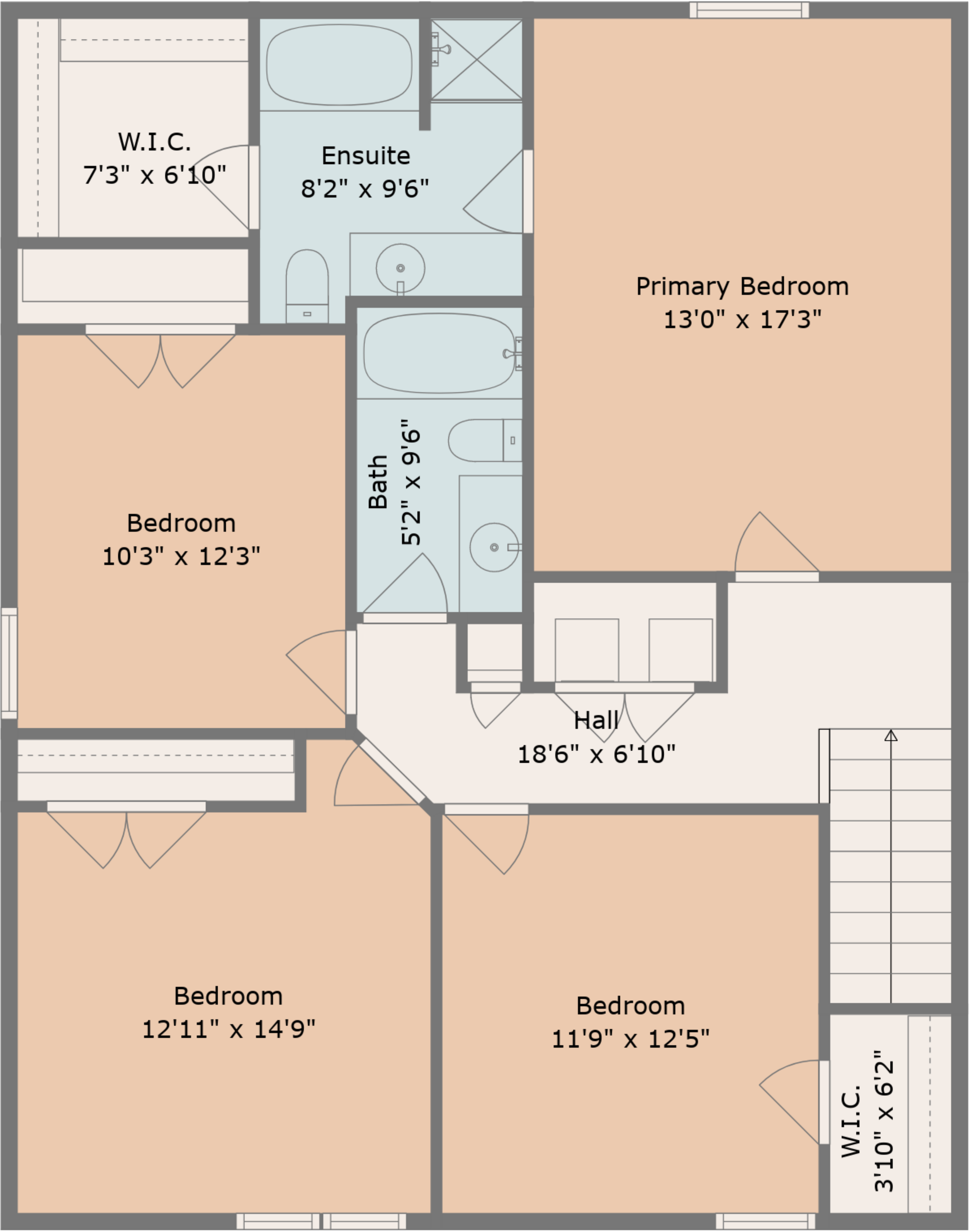
Floor 2
