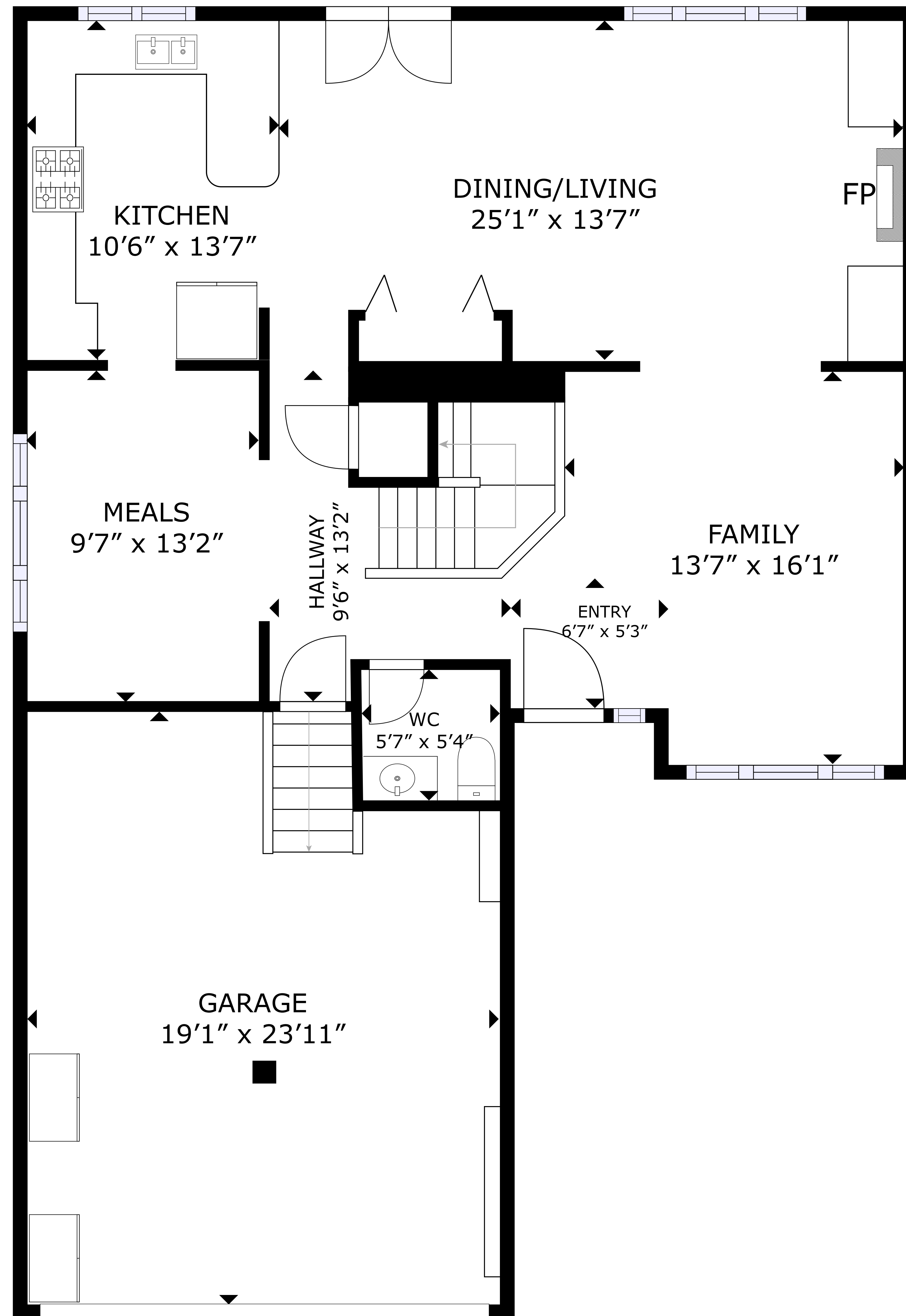
1ST FLOOR
