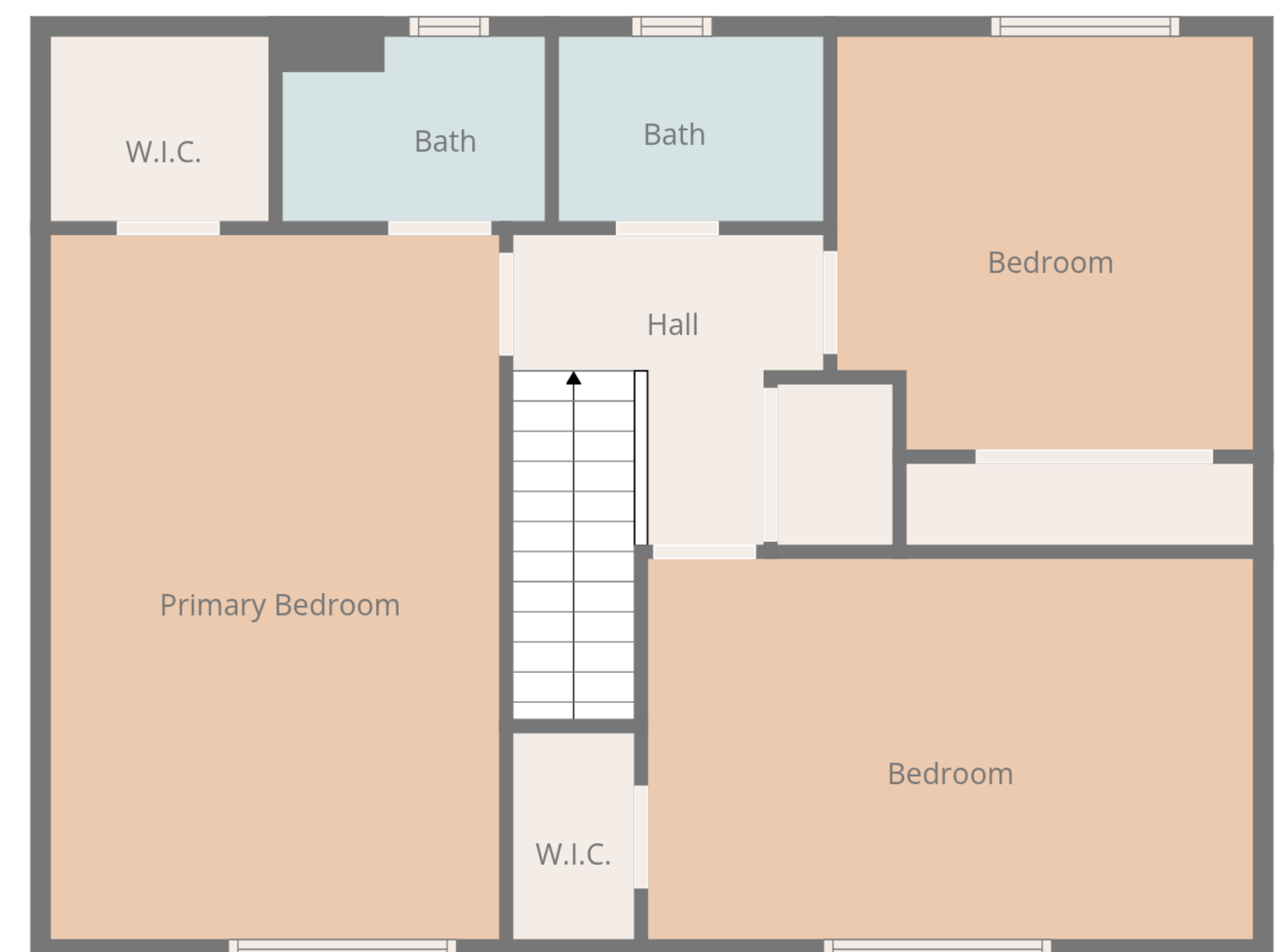
Floor 3
