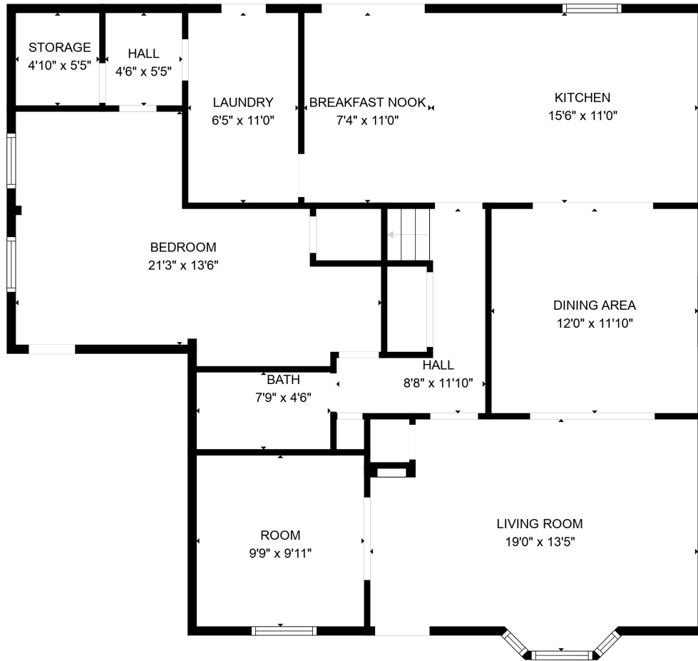
FLOOR 1
