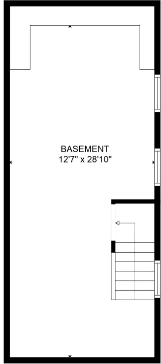
FLOOR 1
