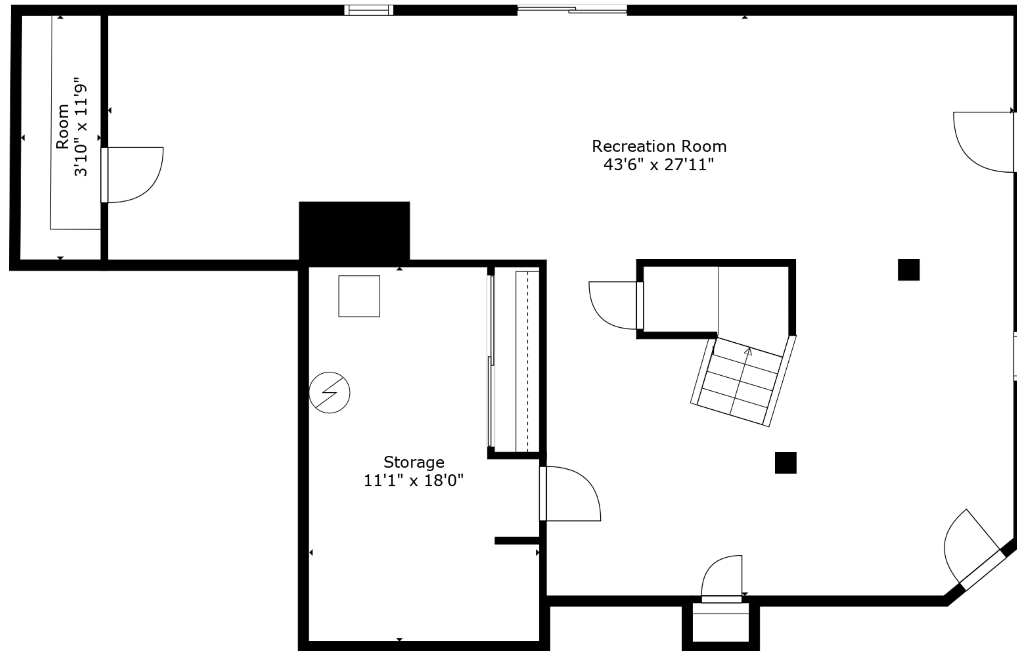
Floor 1
