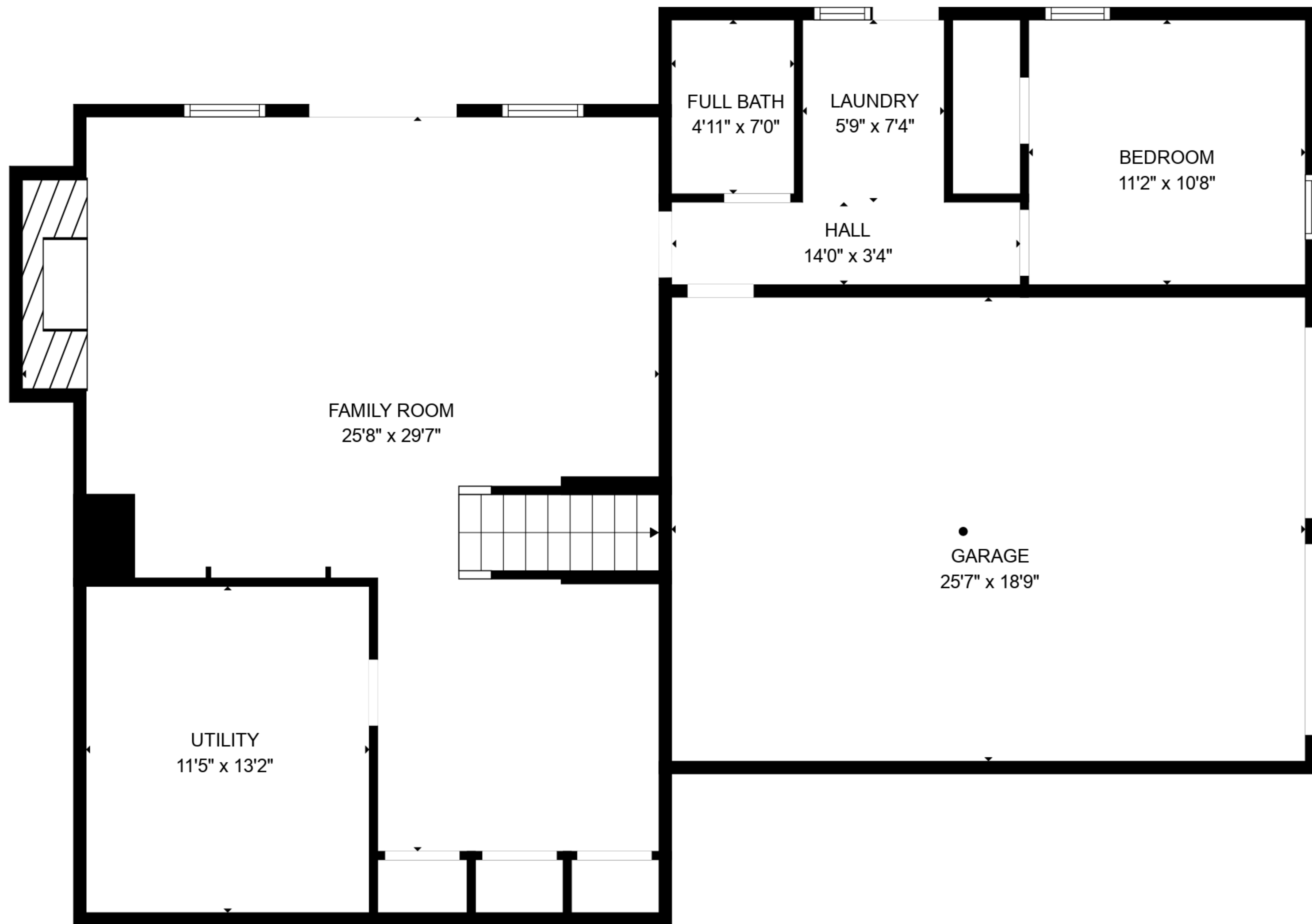
LOWER LEVEL
