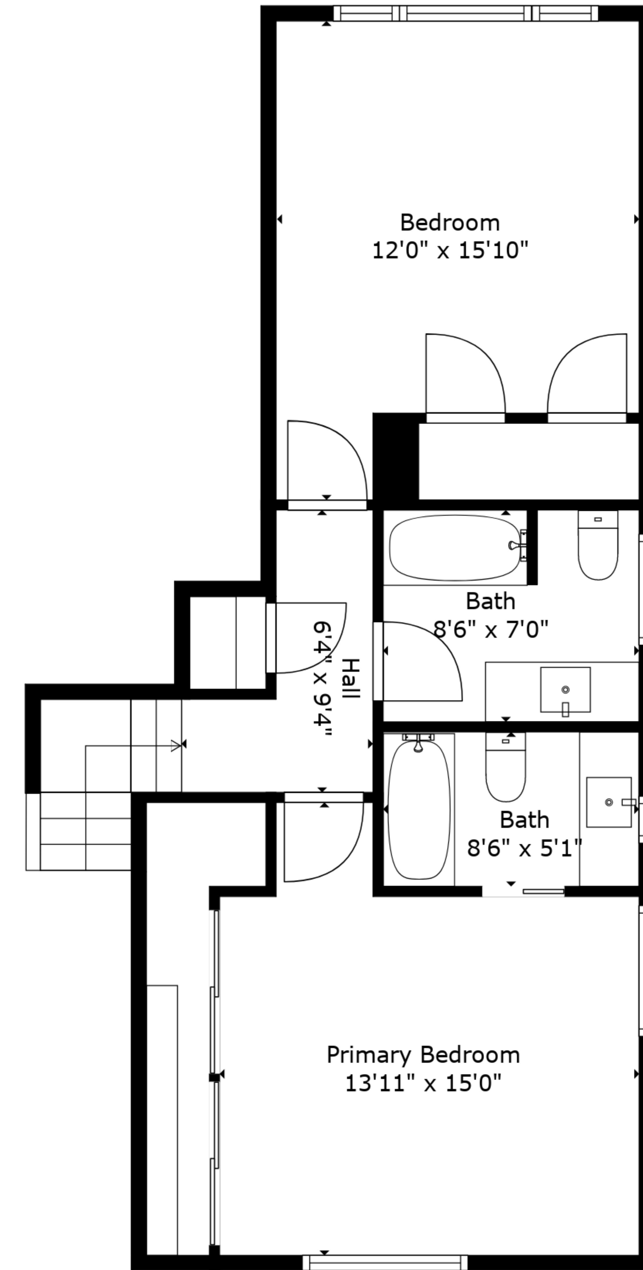
Floor 3
