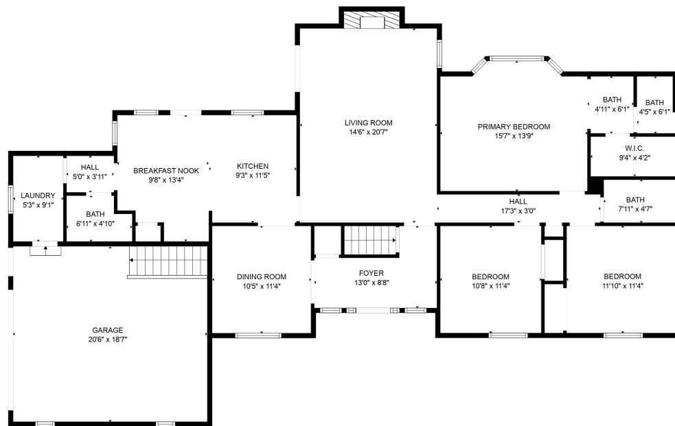
FLOOR 2
