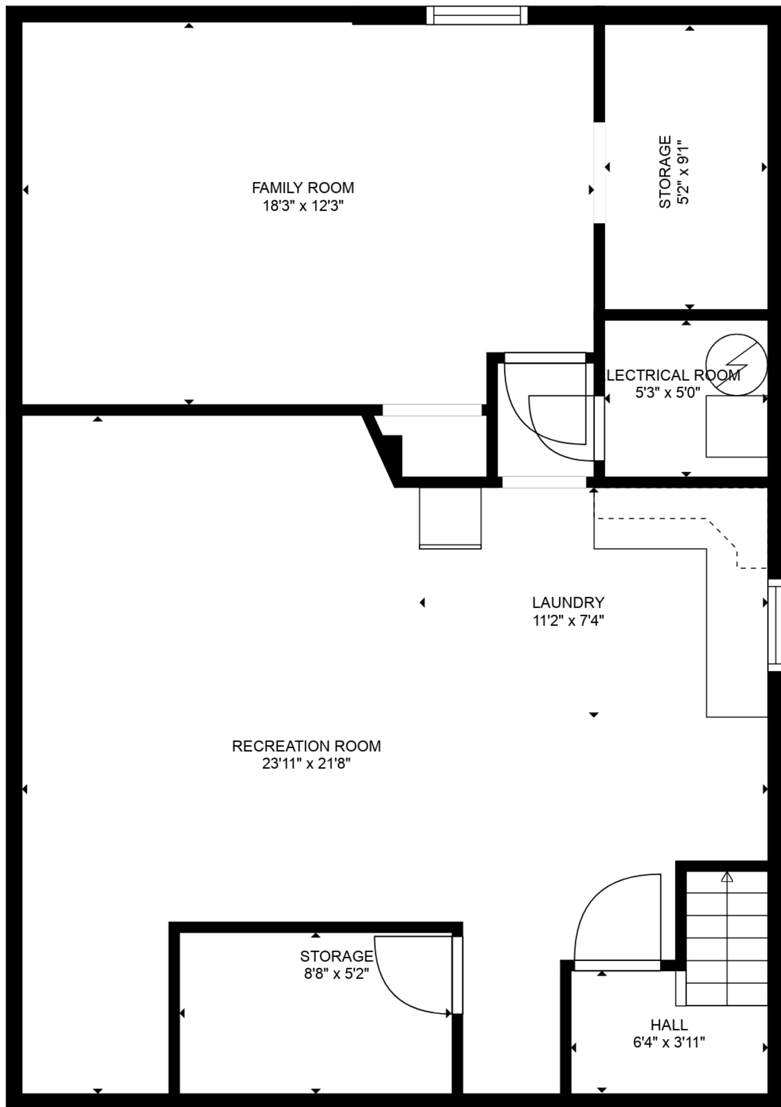
FLOOR 1
