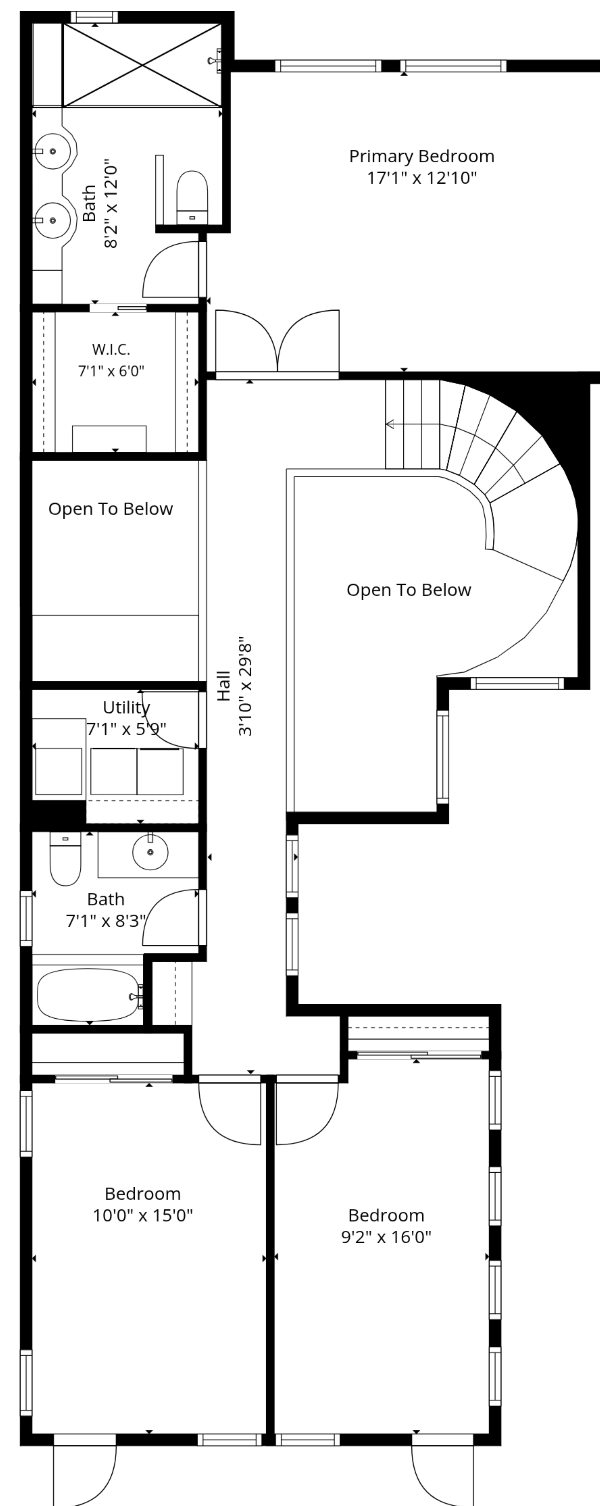
2nd Floor
