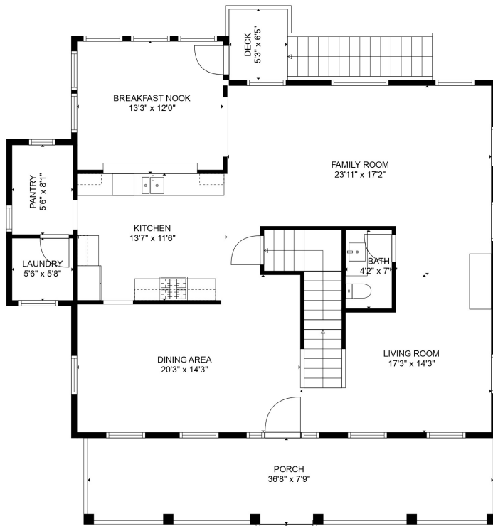
FLOOR 2
