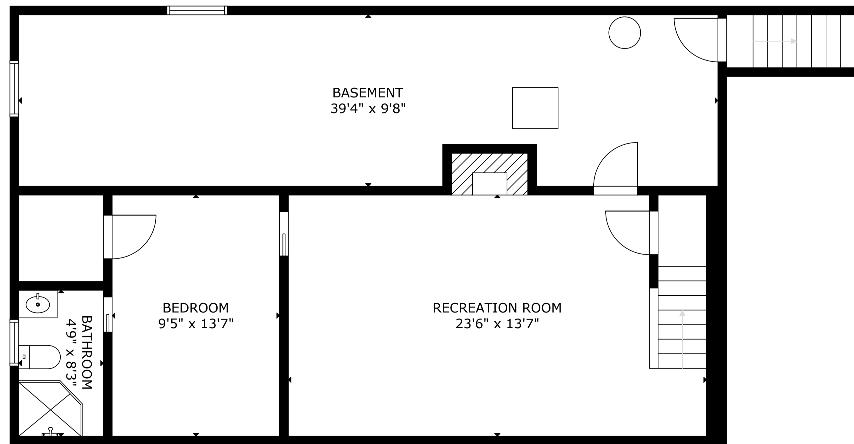
LOWER FLOOR
